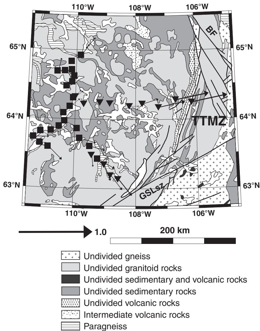
Figure 3. Real (reversed) induction arrows at 100 s on a bedrock map of the area. Unit vector shown. TTMZ, Thelon–Talston magmatic zone; GSLsz, Great Slave Lake shear zone; filled inverted triangles, MT sites for Walmsley Lake project experiment; filled squares, MT winter road sites recorded in March 1998, 1999, and 2000
