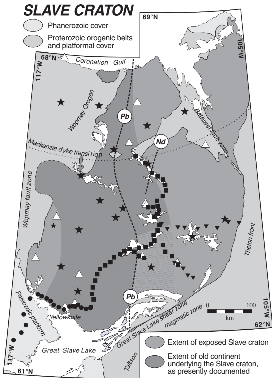
Figure 1. Map of the Slave craton from Bleeker et al. (1999) showing the locations of teleseismic and magnetotelluric sites. Filled dots, MT sites recorded during SNORCLE 1996; filled squares, MT winter road sites recorded in March 1998, 1999, and 2000; filled stars, ocean-bottom MT instrumentation deployed during 1998–1999 and 1999–2000; filled inverted triangles, MT sites for Walmsley Lake project experiment; open triangles, teleseismic sites of Bank et al. (2000); dark grey is the documented extent of the Central Slave Basement Complex (Bleeker et al. 1999), and the lighter grey region is its presumed extension beneath the Walmsley Lake area. Also shown are the isotope boundaries (Pb and Nd).
