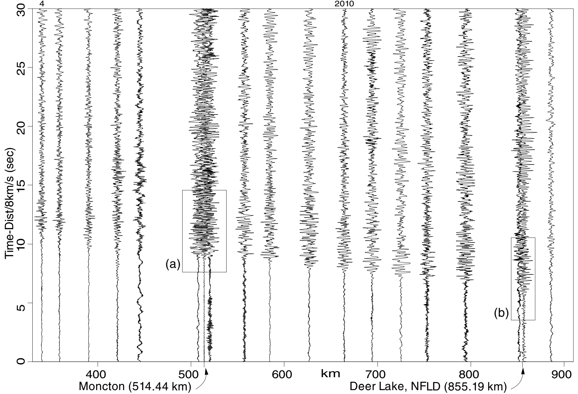
CPF Shock Trial #825 data; 340-900 km, PRS (unfiltered) and Standard Station (>4hz)
