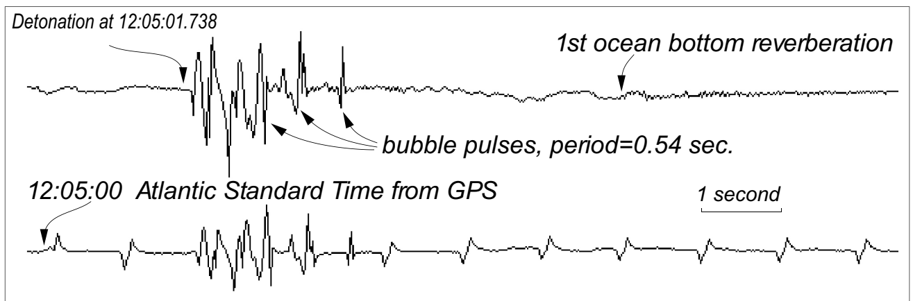
CPF Shock Trial OBS record from the bridge of HMCS Halifax November 18, 1994
