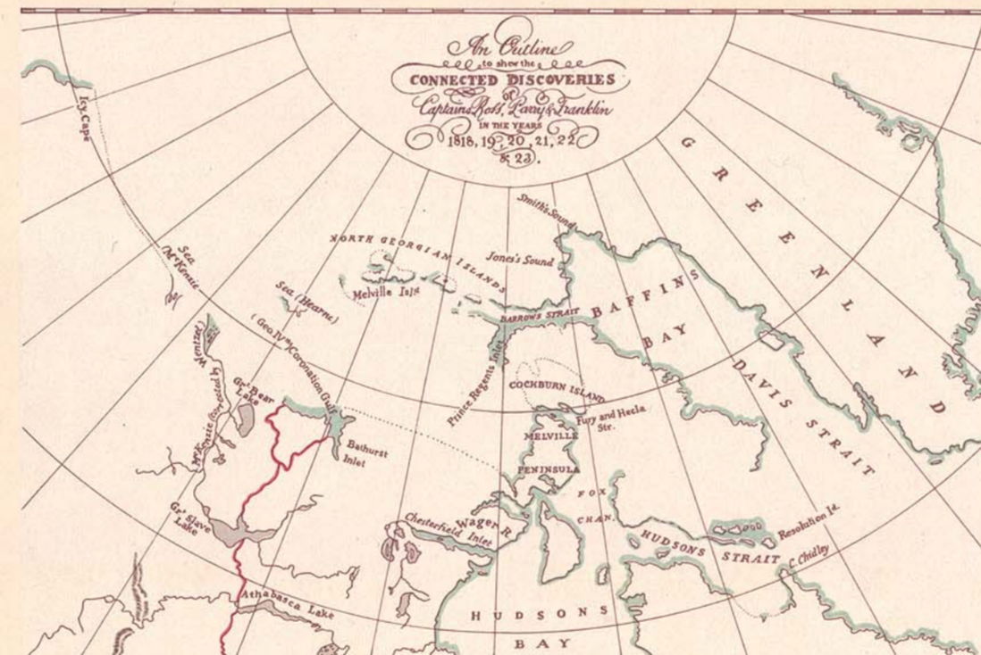
Franklin 1823
