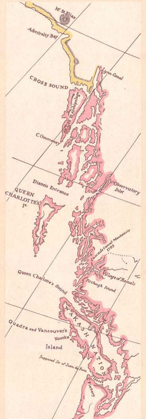
Arrowsmith 1822
