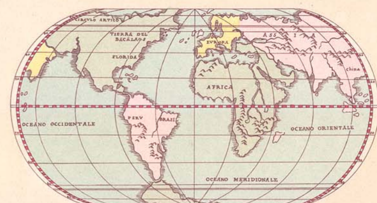
Ptolemy, 1548 Edition
