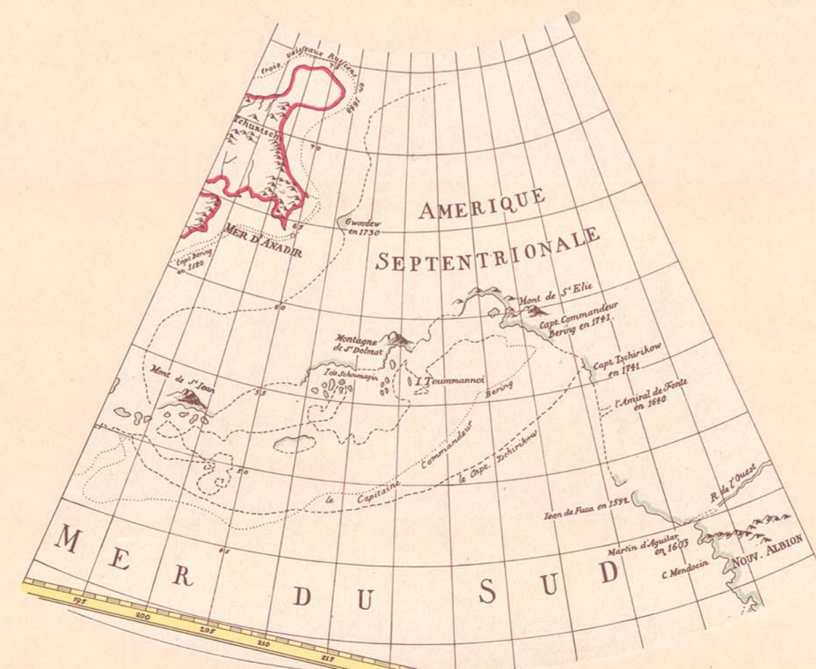
Anonymous 1758
