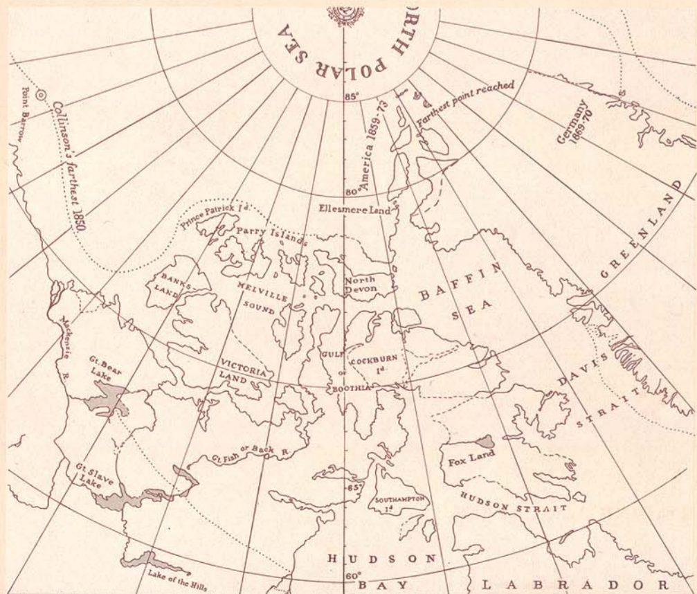
British Admiralty 1874
