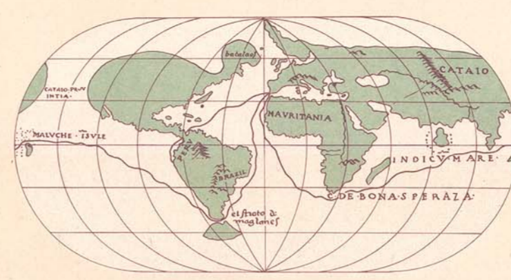
Agnese 1540
