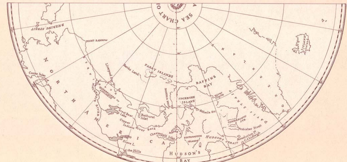
British Admiralty 1835
