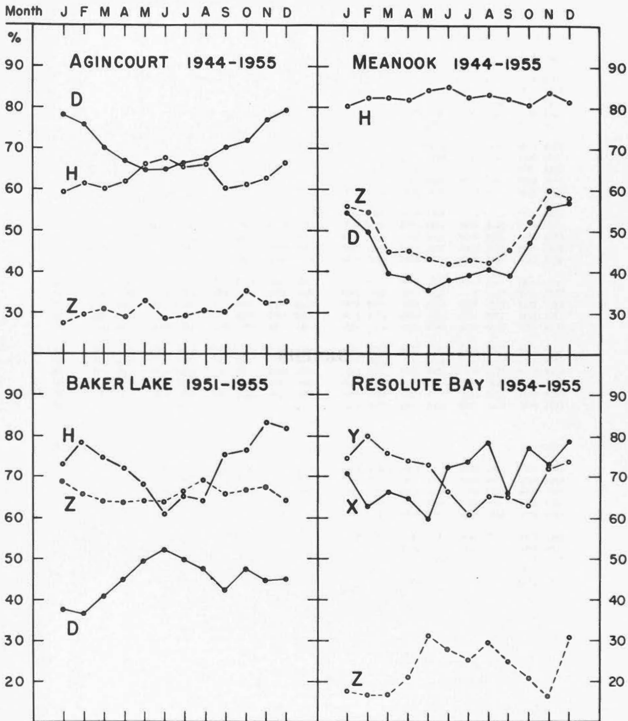
The percent of the total number of three-hour intervals during a given month over a period of years that an element could supply the K-index value.
