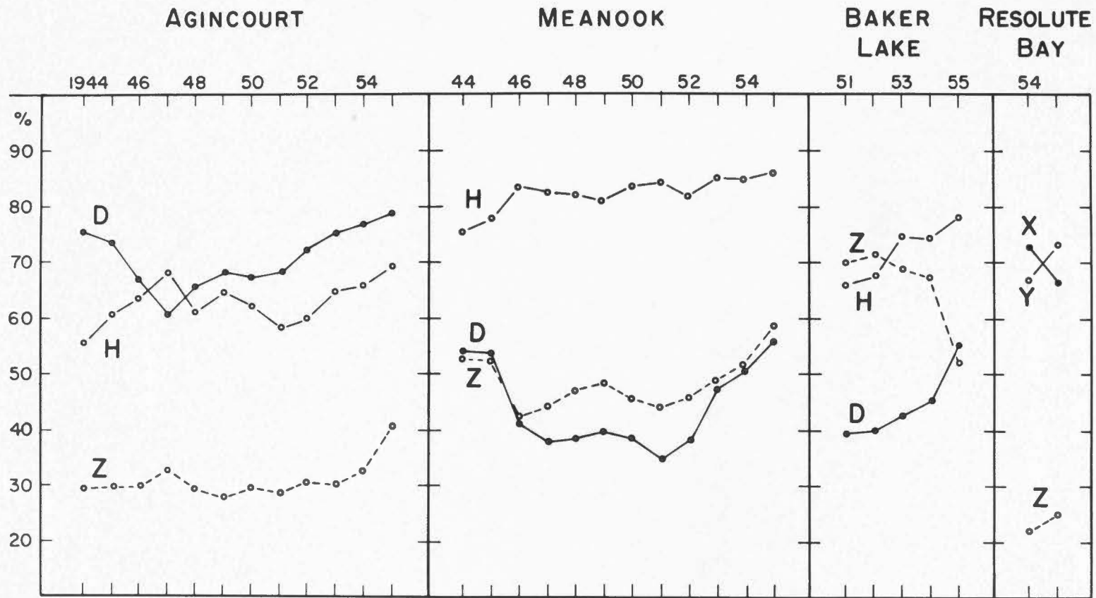
The percent of the total number of three-hour intervals during a given year that an element could supply the K-index value.
