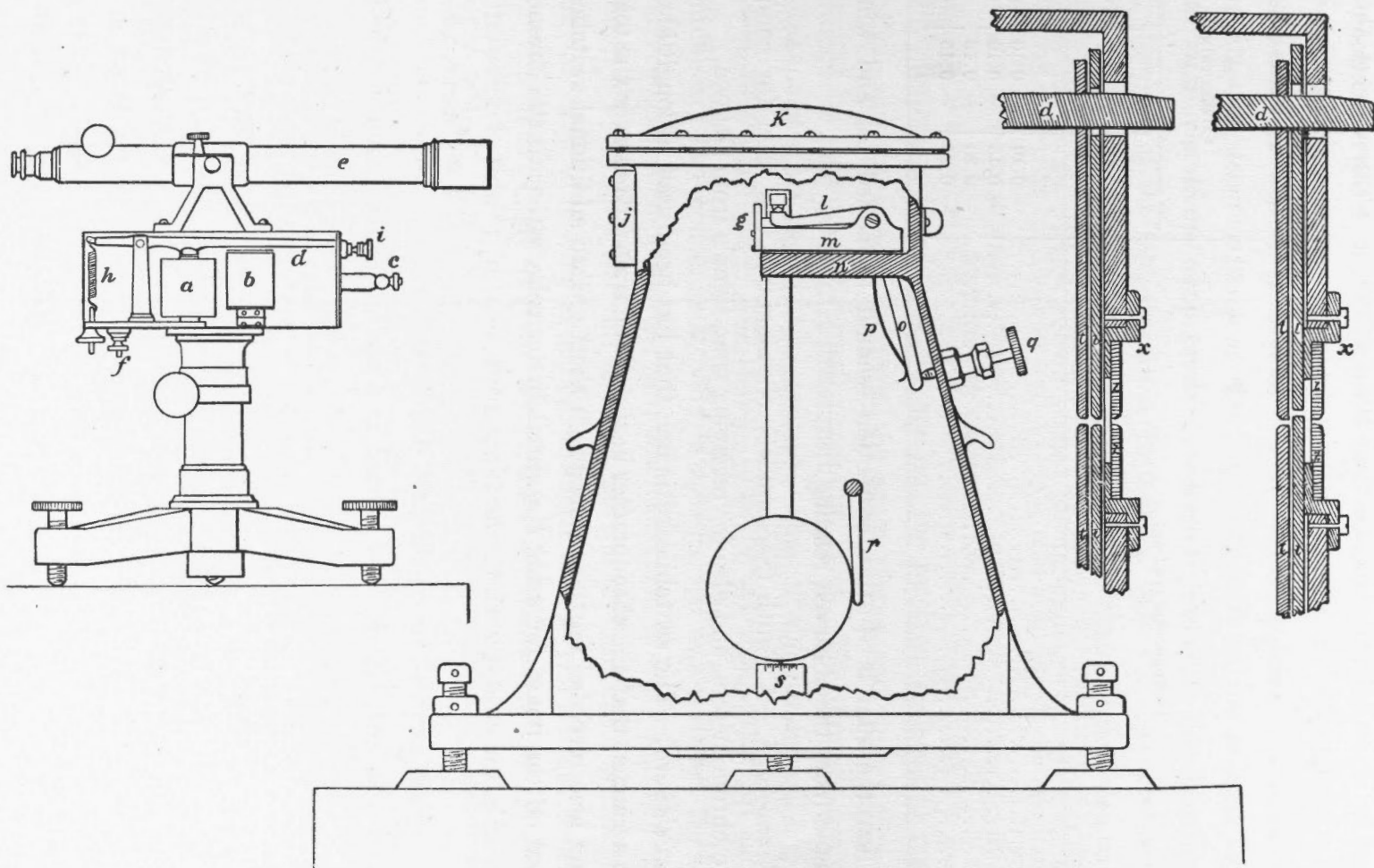
FIG. 1.—SIDE ELEVATION OF RECEIVER AND FLASH APPARATUS AND SECTION THROUGH SHUTTERS.
