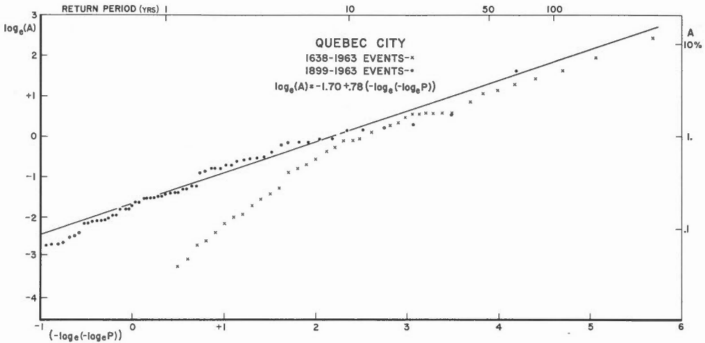
Figure 5. Extreme value distribution plot for Quebec City.
