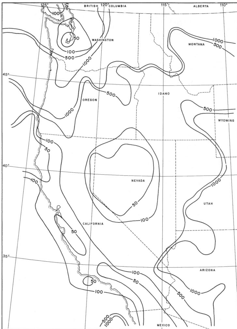
Figure 9. Return periods in years for acceleration of 10 per cent gravity for western United States.
