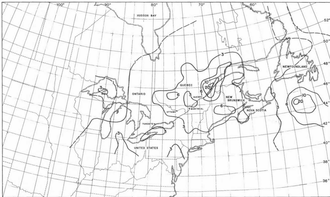
Figure 6. Accelerations as a per cent of g with a 100-year return period for eastern Canada.
