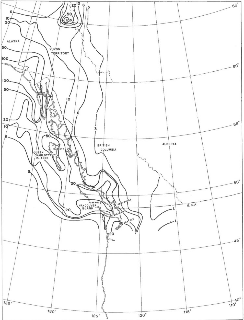
Figure 8. Accelerations as a per cent of g with a 100-year return period for western Canada.
