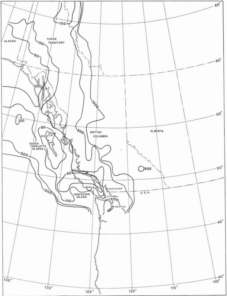
Figure 7. Return periods in years for acceleration of 10 per cent gravity in western Canada.
