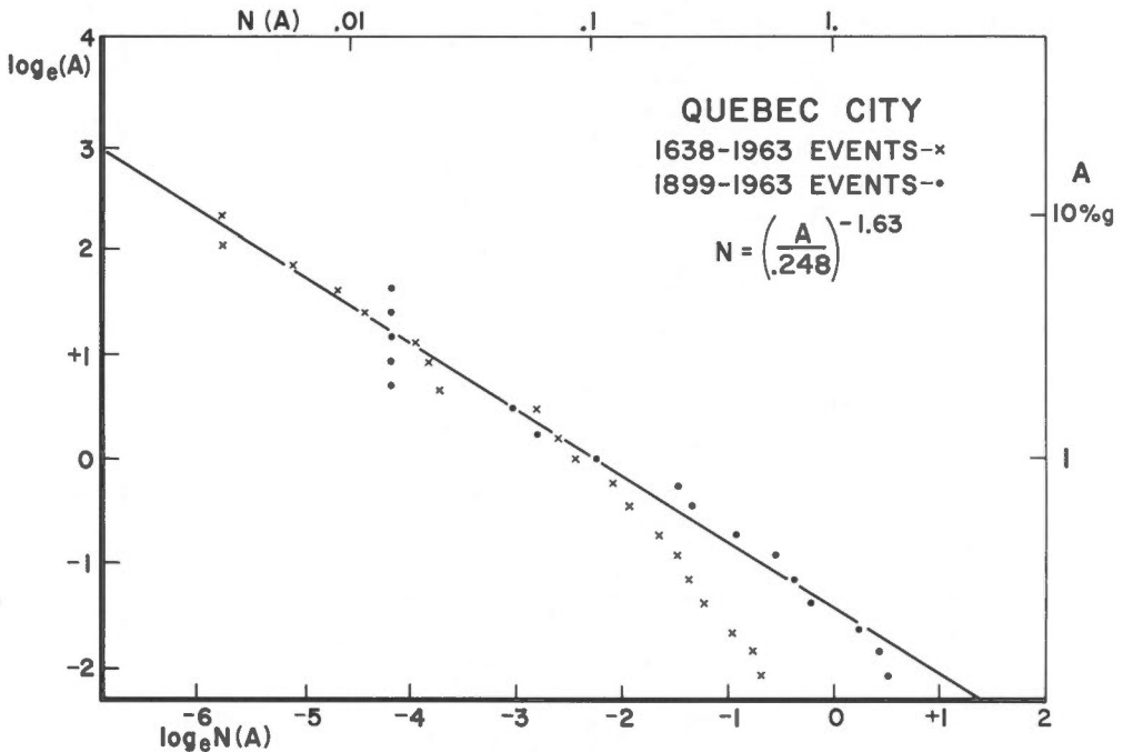
Figure 3. Average distribution plots for Quebec City.
