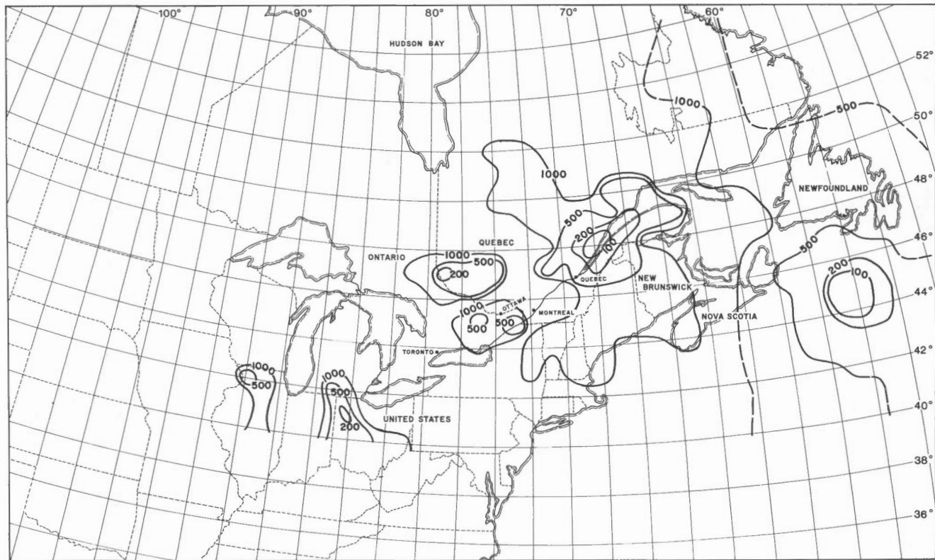
Figure 4. Return periods in years for acceleration of 10 per cent gravity in eastern Canada.
