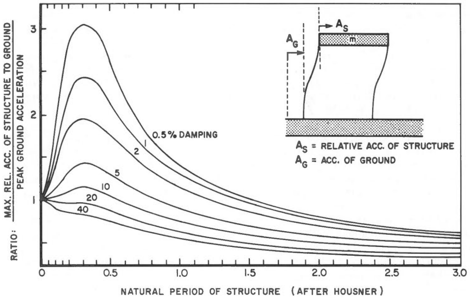
Figure 11. Earthquake acceleration response spectrum (after Housner).
