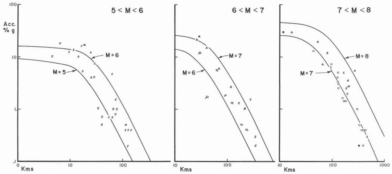
Figure 1. Relationship between acceleration and distance in western North America.
