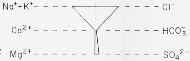
FIGURE 23 REGINA-MOOSE JAW AREA REPRESENTATIVE STIFF DIAGRAMS OF SUBSURFACE WATERS
