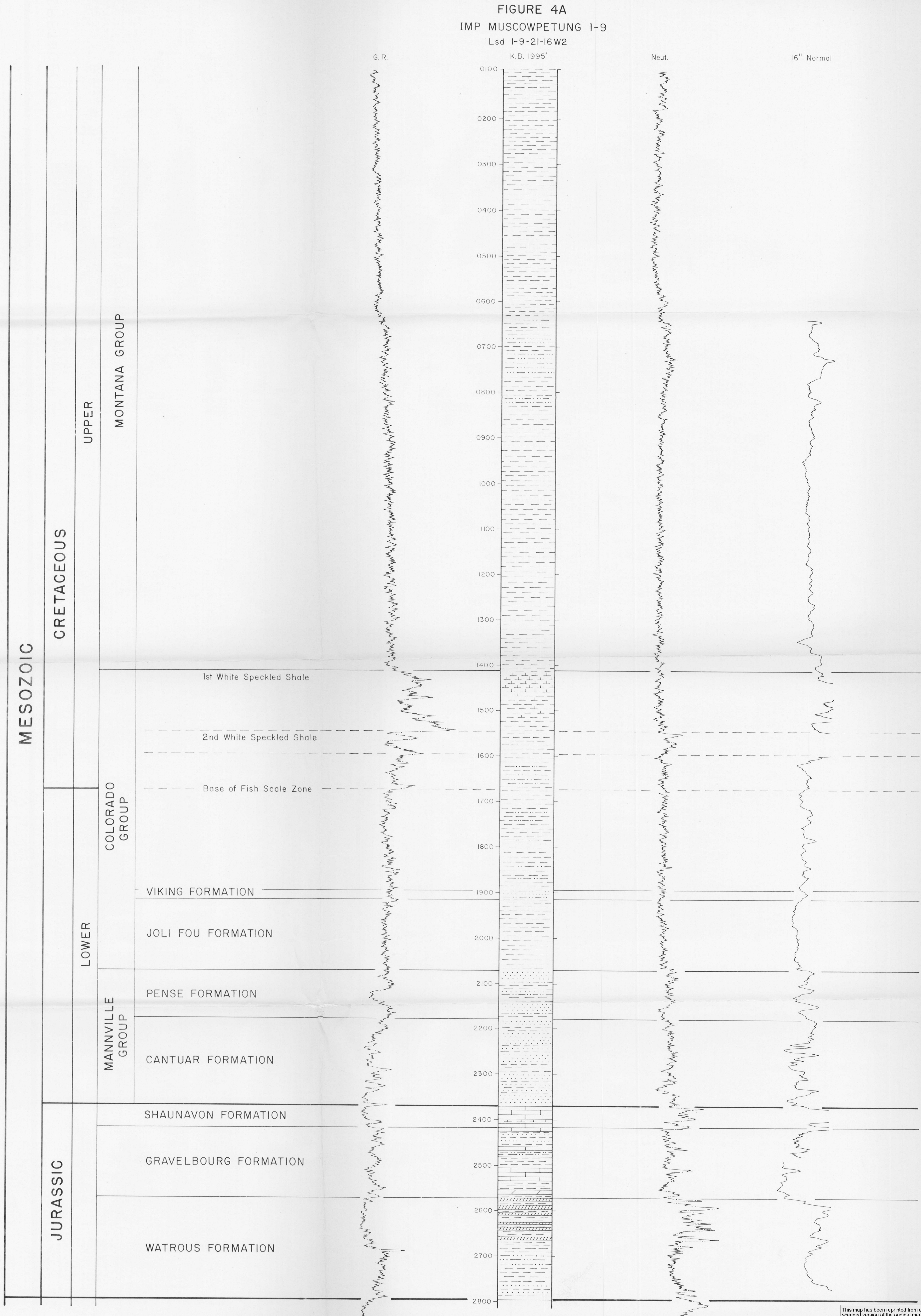
FIGURE 4 REFERENCE WELL FOR THE REGINA-MOOSE JAW AREA SASKATCHEWAN
