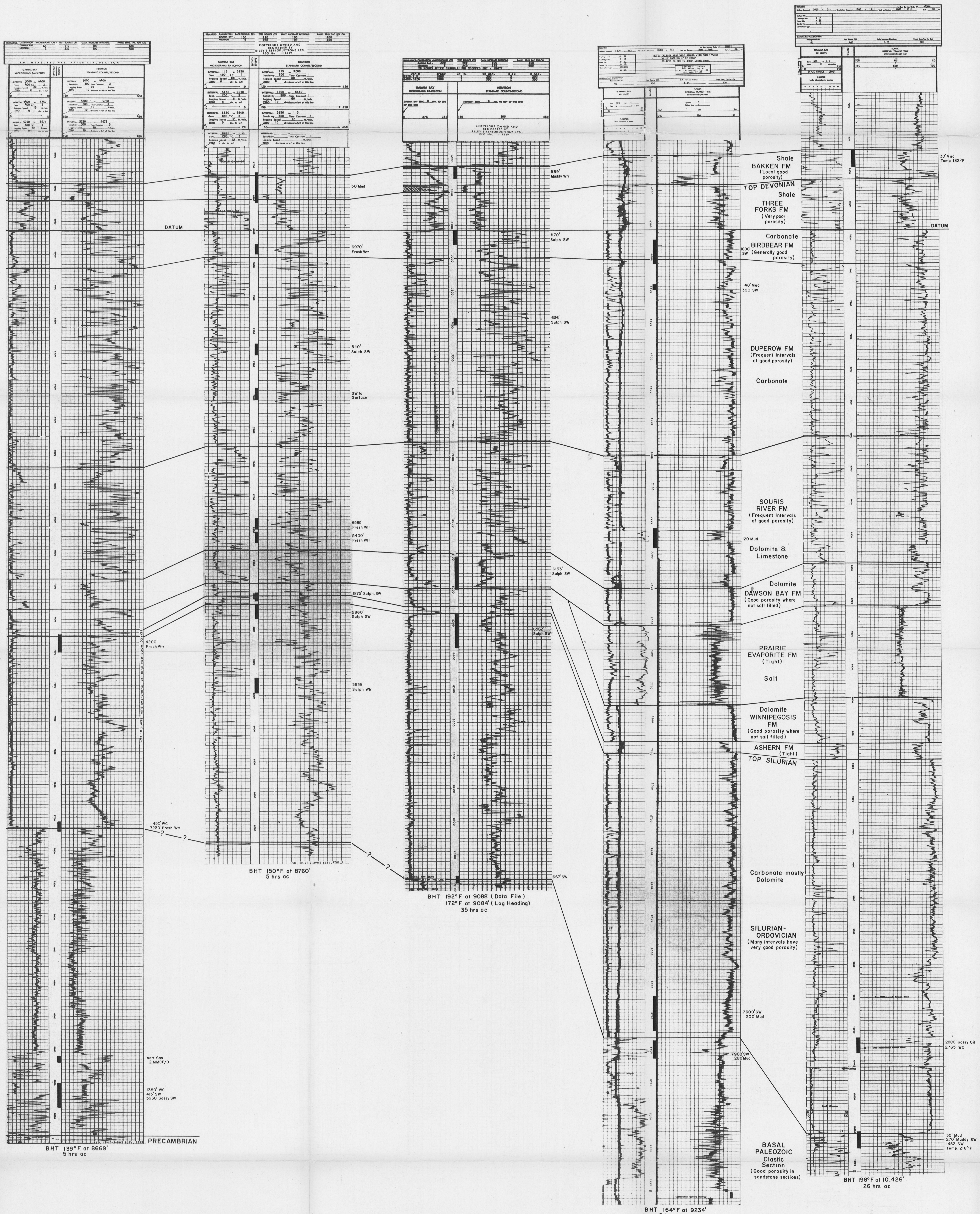
FIGURE - 3 CROSS SECTION A-A' SOUTH CENTRAL SASKATCHEWAN
