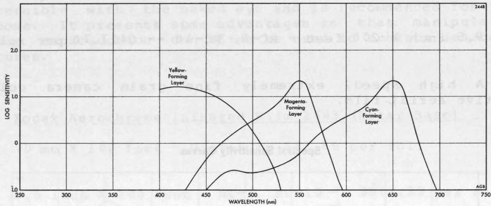
Figure 11 -- 2448 Spectral Sensitivity
