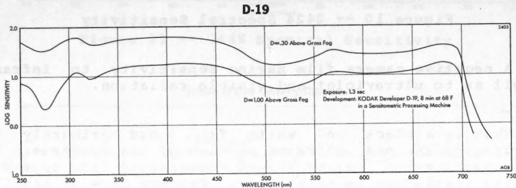
Figure 9 -- 2405 Spectral Sensitivity
