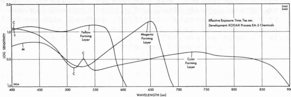
Figure 15 -- 2443 Spectral Sensitivity
