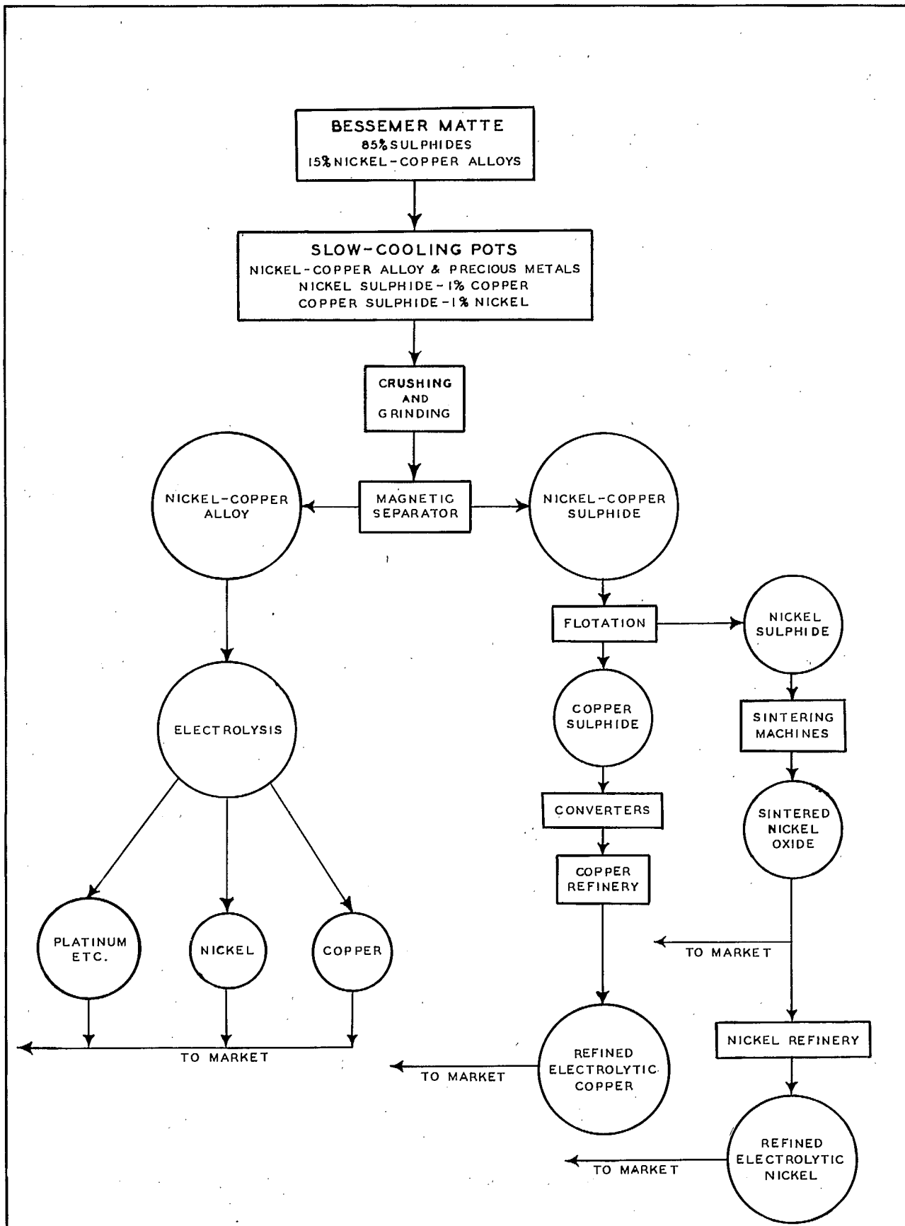
FIGURE I. MATTE FLOTATION PROCESS
