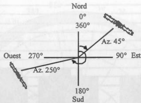
Figure 2.12 Azimut
