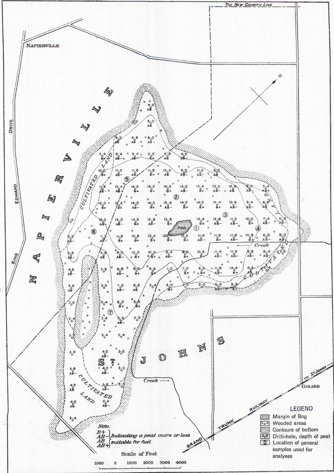
GIRARD PEAT BOG, ST. JOHNS AND NAPIERVILLE COUNTIES, QUE.
