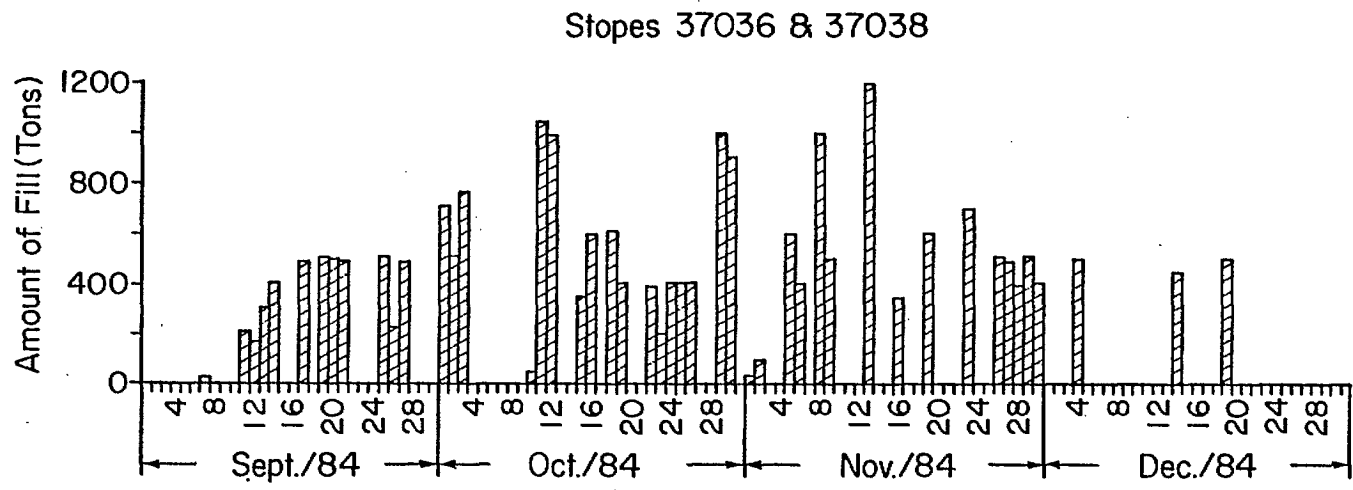
Fig. 4 - Amount of backfill poured in experimental stopes.
