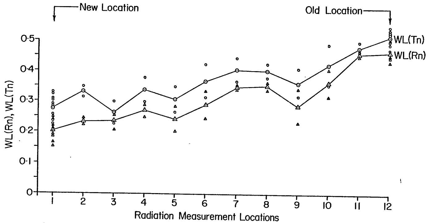
Fig. 15 - Grab-sampling measurements taken at 12 different locations along the 35950 travelway.
