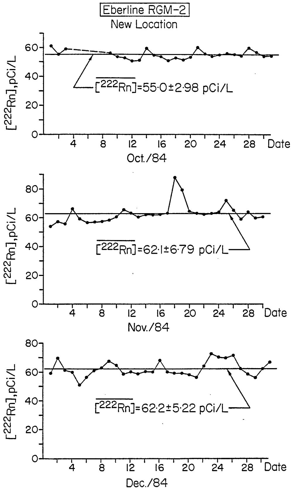
Fig. 19 - Radon gas concentration (new location) versus time and the monthly average values.
