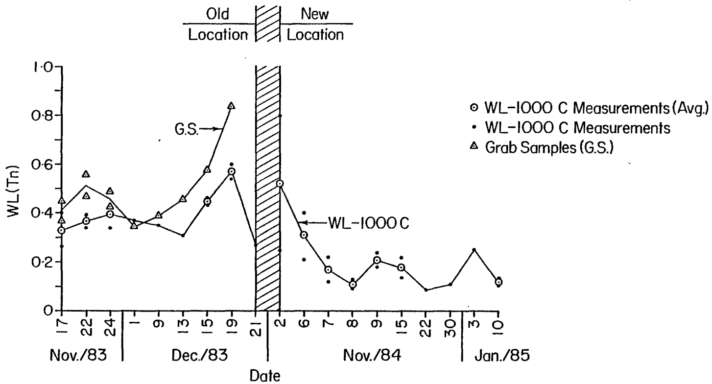
Fig. 13 - WL(Tn) as a function of time (new and old locations).
