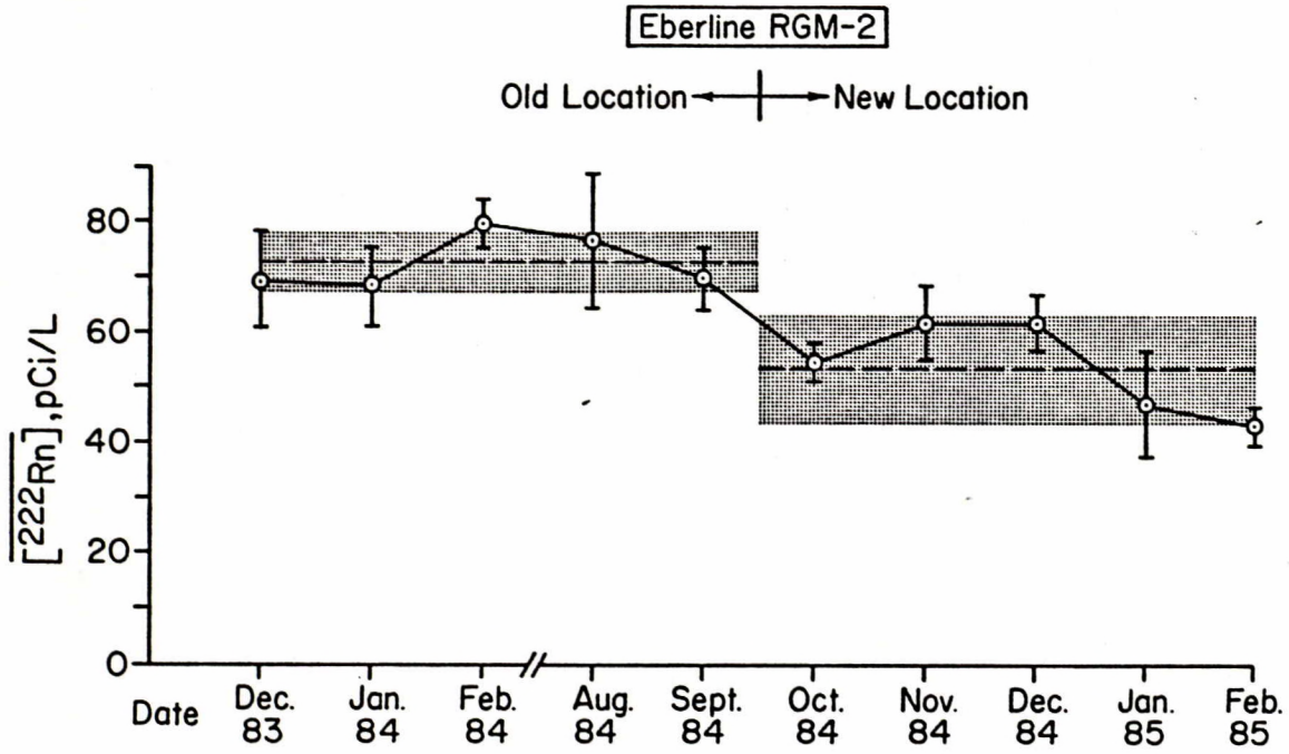
Fig. 21 - Radon gas concentration (monthly average) for the old and new locations.
