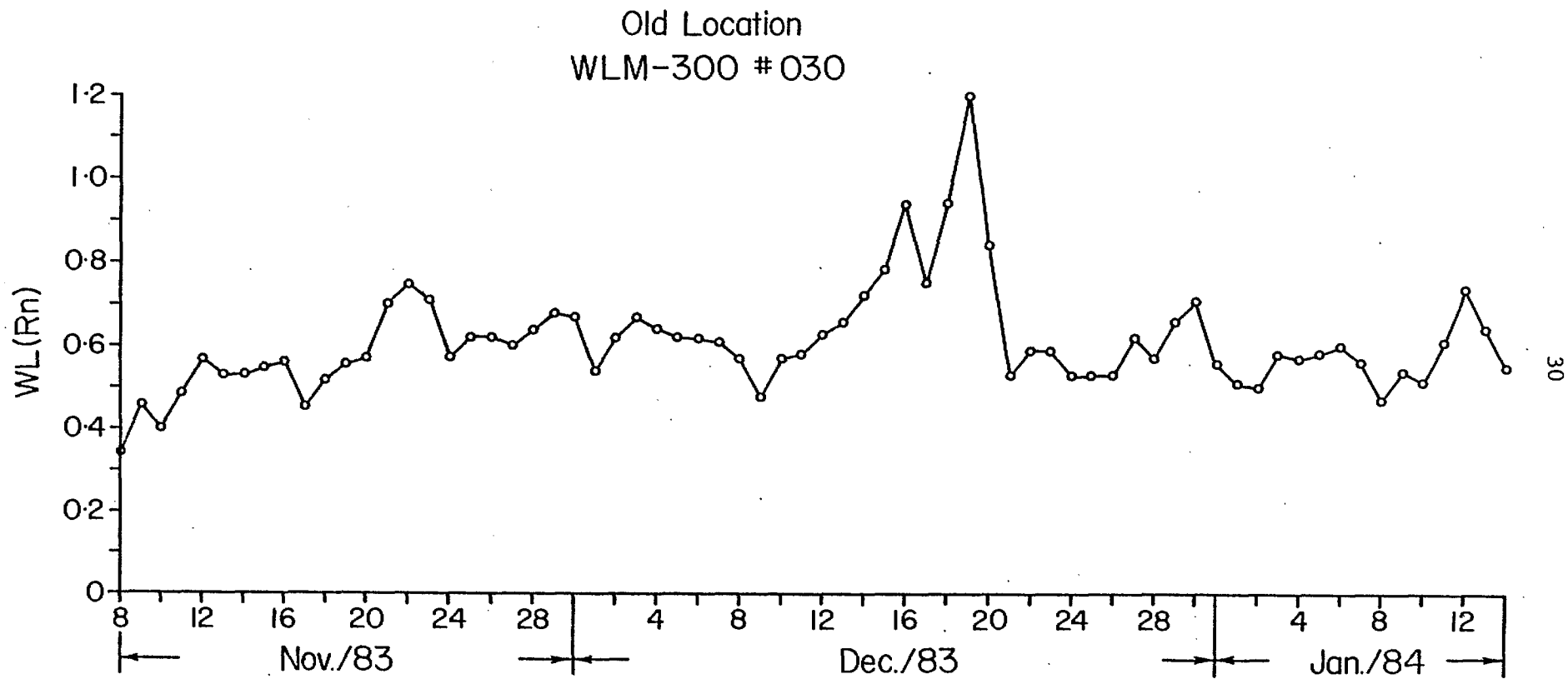
Fig. 10 - WL(Rn) as a function of time (old location).
