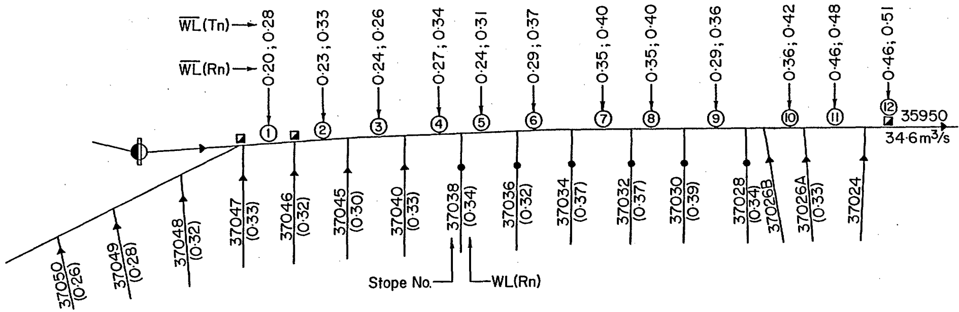
Fig. 16 - Grab-sampling measurements taken at 12 different locations along the 35950 travelway.
