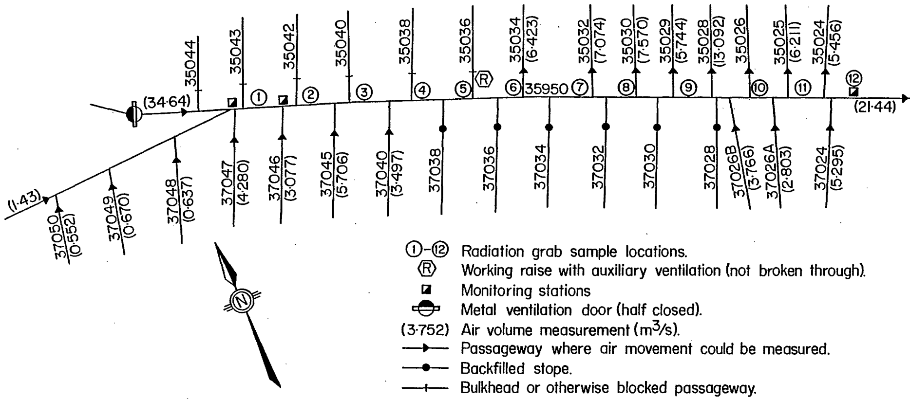
Fig. 2 - Ventilation survey data in the general U/G backfill area.
