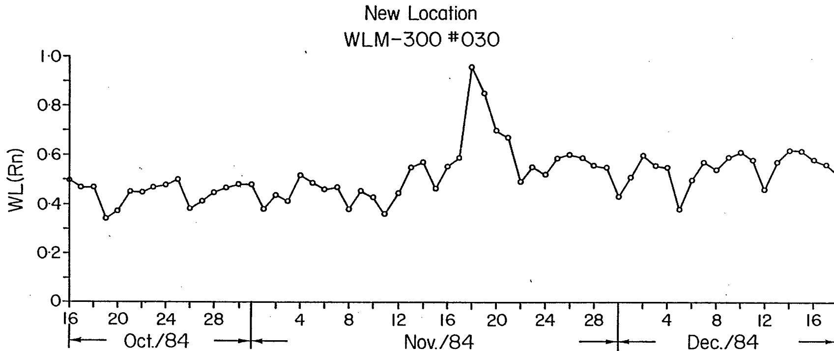
Fig. 12 - WL(Rn) as a function of time (new location).
