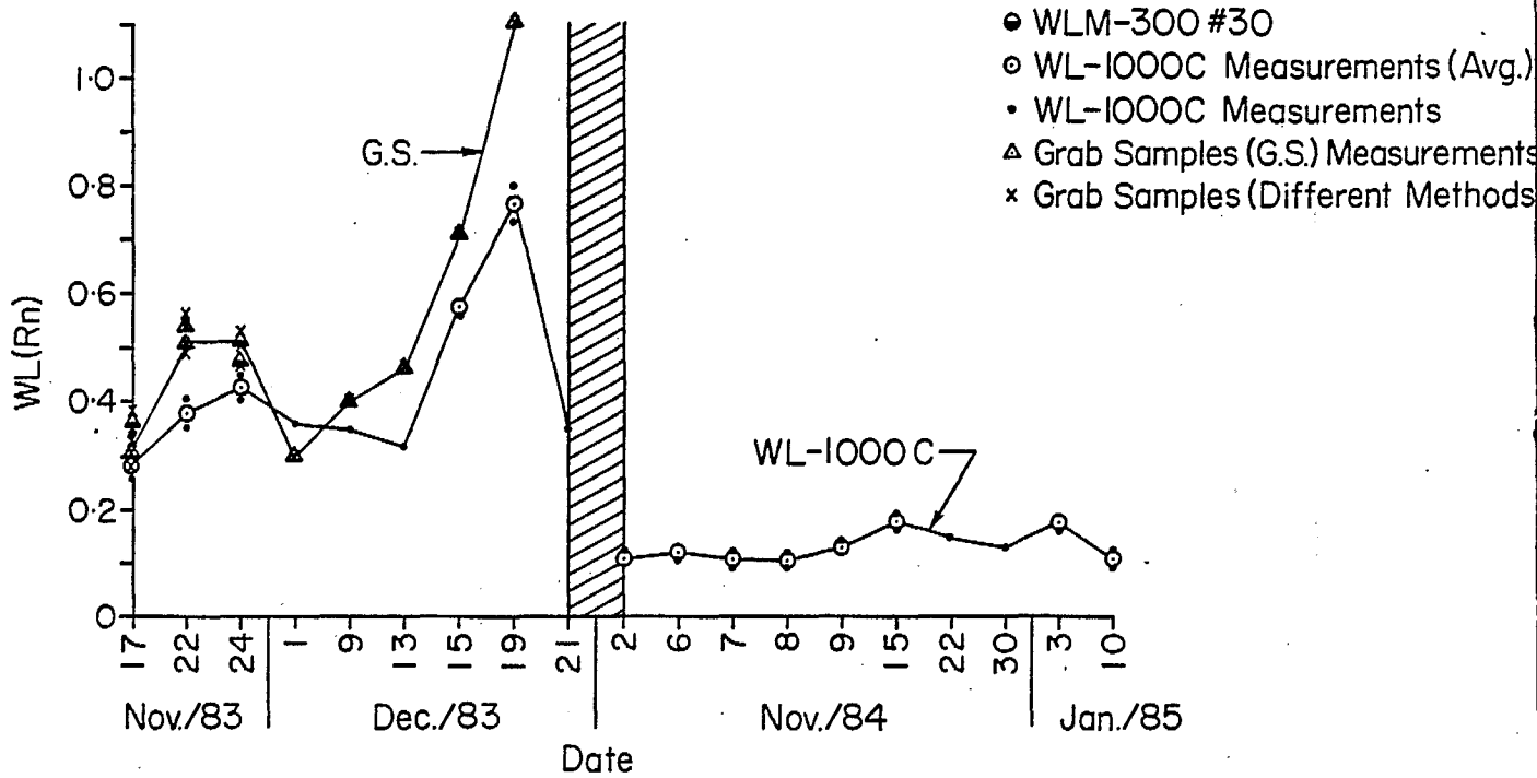
Fig. 14 - WL(Rn) as a function of time (old and new locations).
