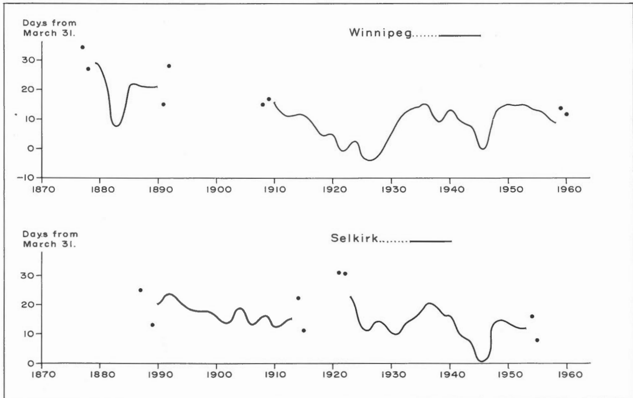
FIGURE 21. 5-point filtered series of break-up.
