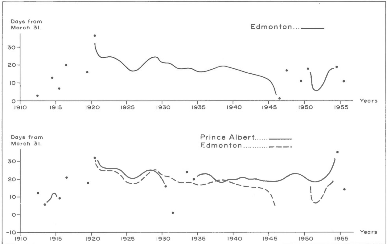
FIGURE 2. 5-point filtered series of last-ice.
