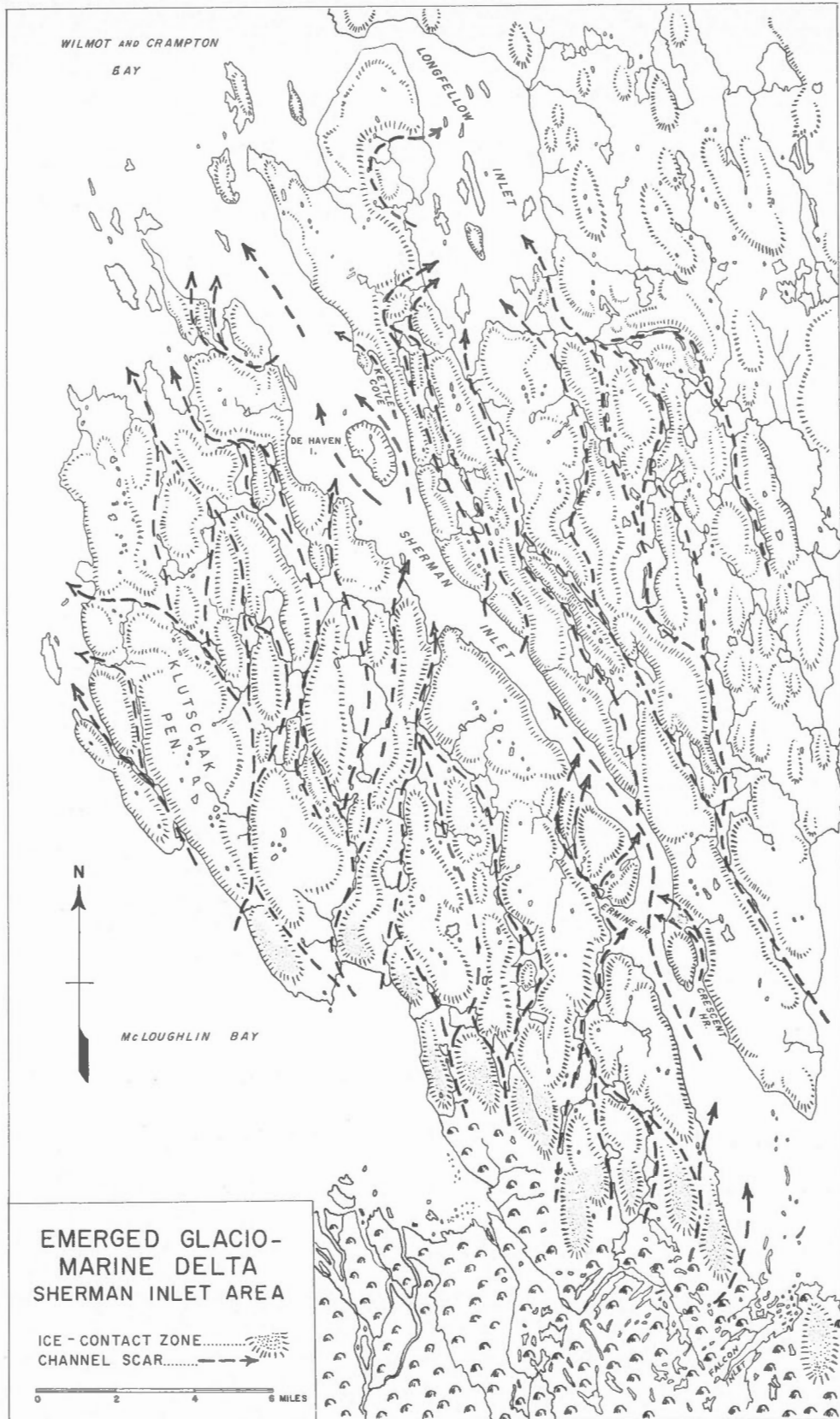
Figure 18. Map of Klutschak Peninsula, showing glacial spillways and ice contact face.
