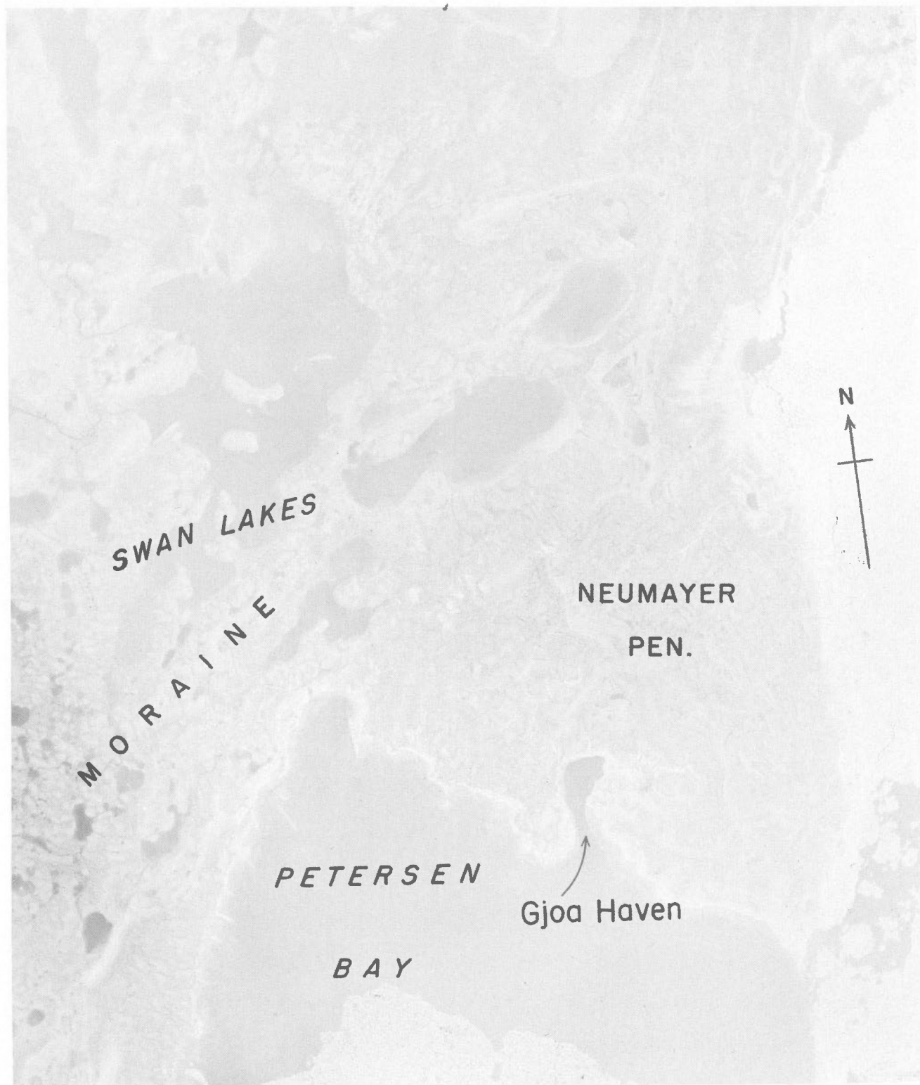
Figure 15. Neumayer Peninsula, King William Island; a vertical photograph taken from 30,000 feet. Gjoa Haven is a kettle in glacio-marine marginal deposits.
