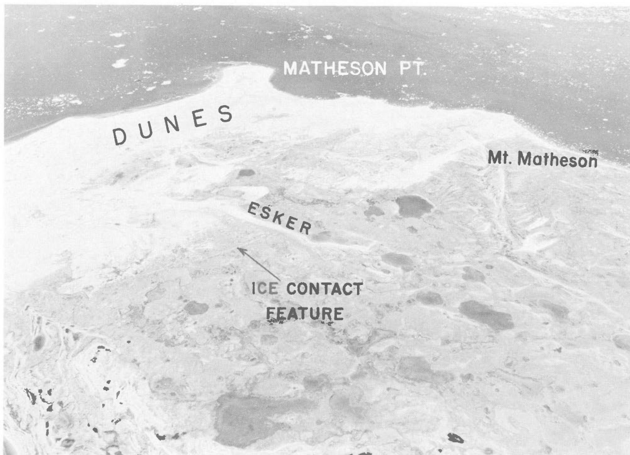
Figure 14. Mount Matheson, King William Island, looking east towards Rae Strait. The eskers and esker delta are crossed by a line speculated to represent the ice margin at the time of the creation of the esker delta.
