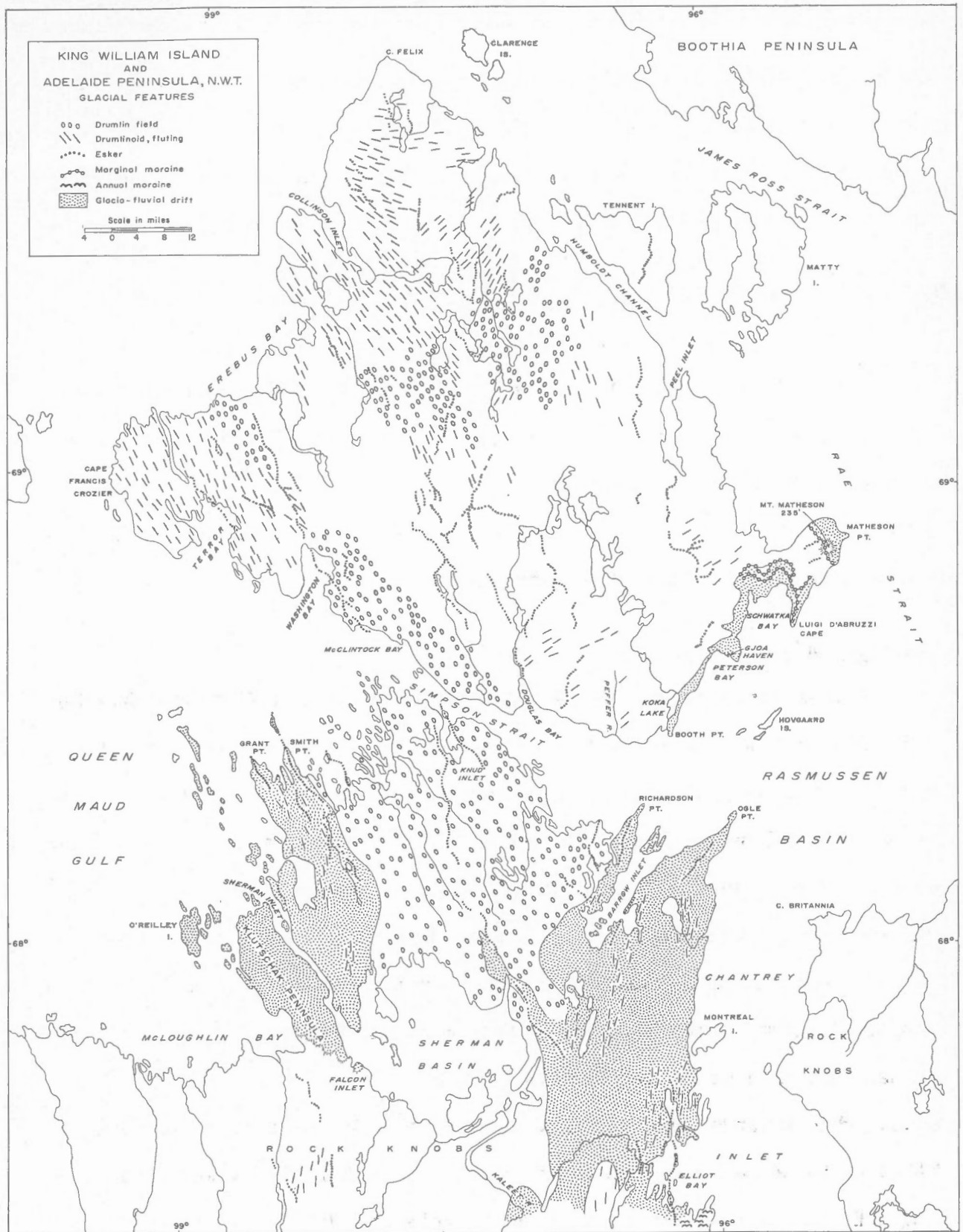
Figure 7. Glacial Features.
