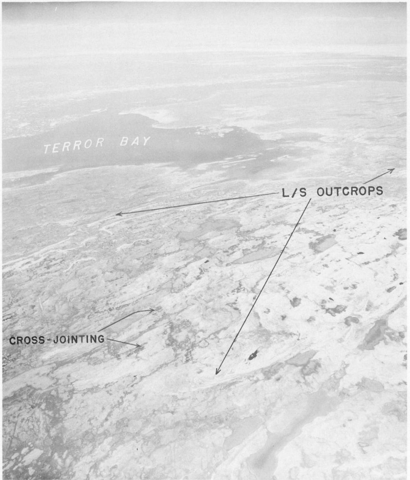
Figure 3. Looking west over Terror Bay, King William Island. Much of the light-toned area is shattered limestone exposures. The cross-jointing pattern appears in the midground and low scarps appear to the left.
