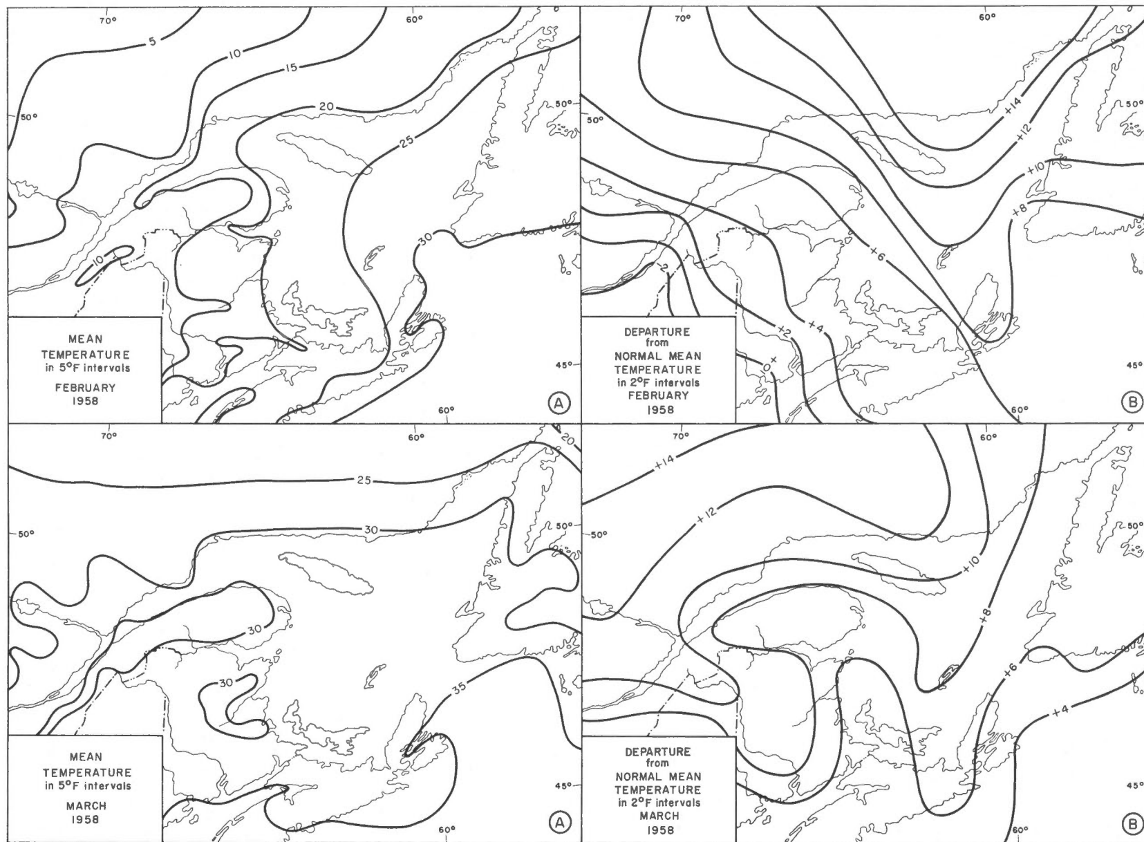
Figure 1. (A) Mean temperatures, December 1957 to March 1958
