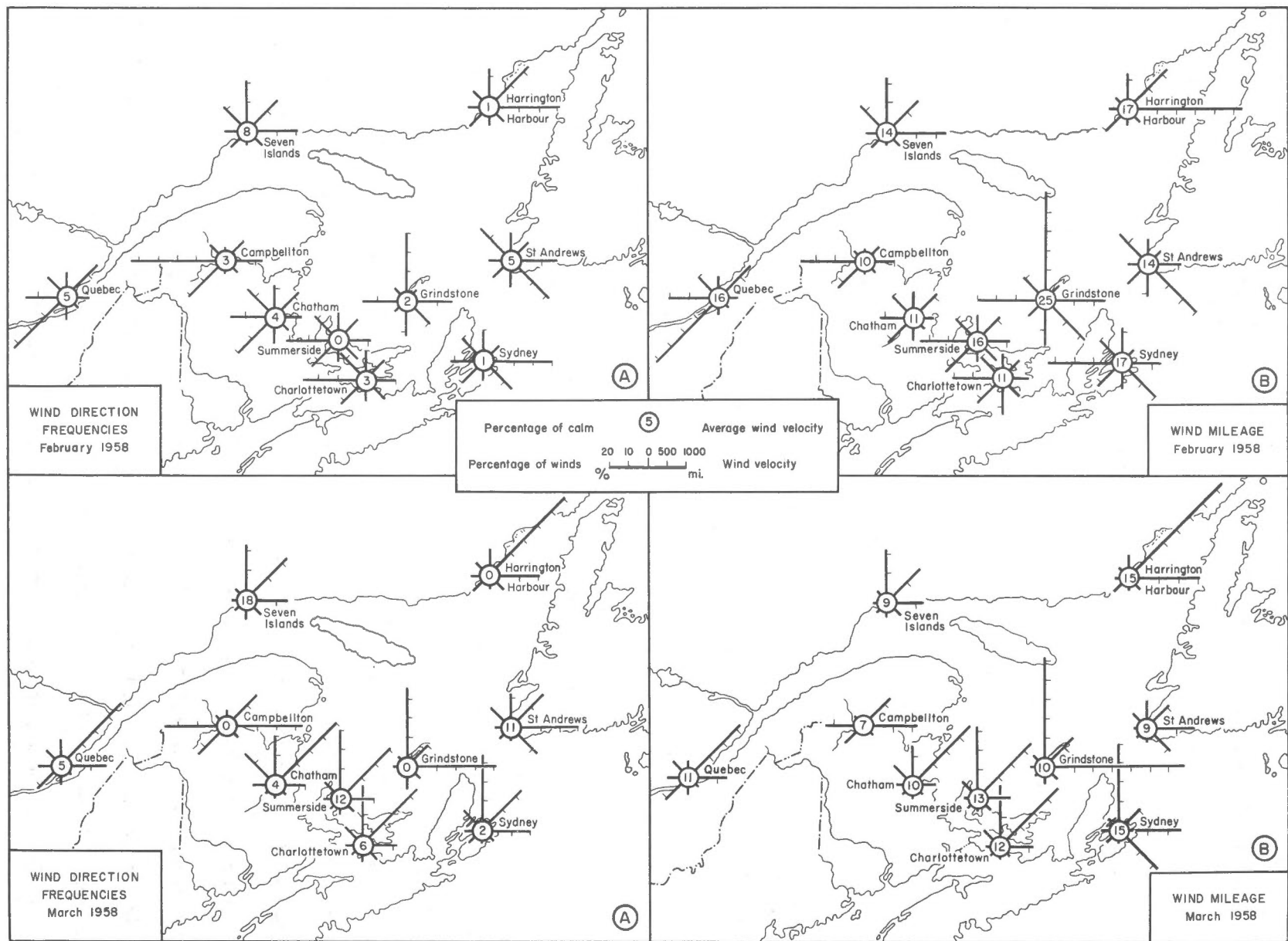
Figure 2. (A) Wind direction frequencies, December 1957 to March 1958 (B) Wind mileage, December 1957 to March 1958
