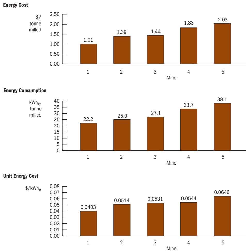
Figure 4.4.4 – Total Energy Costs: Crushing and Grinding Combined
