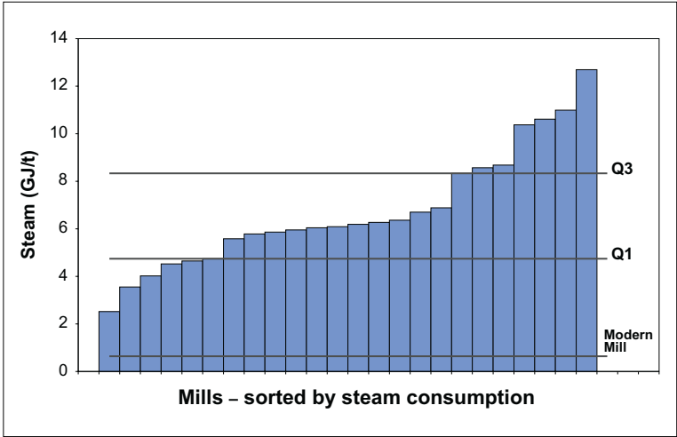
Figure 5. Process steam consumption – newsprint mills
