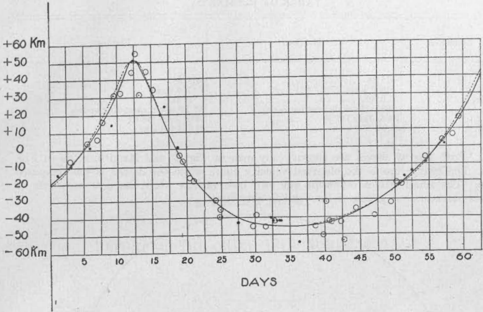
FIG. I.—Velocity Curve of a Draconis.
