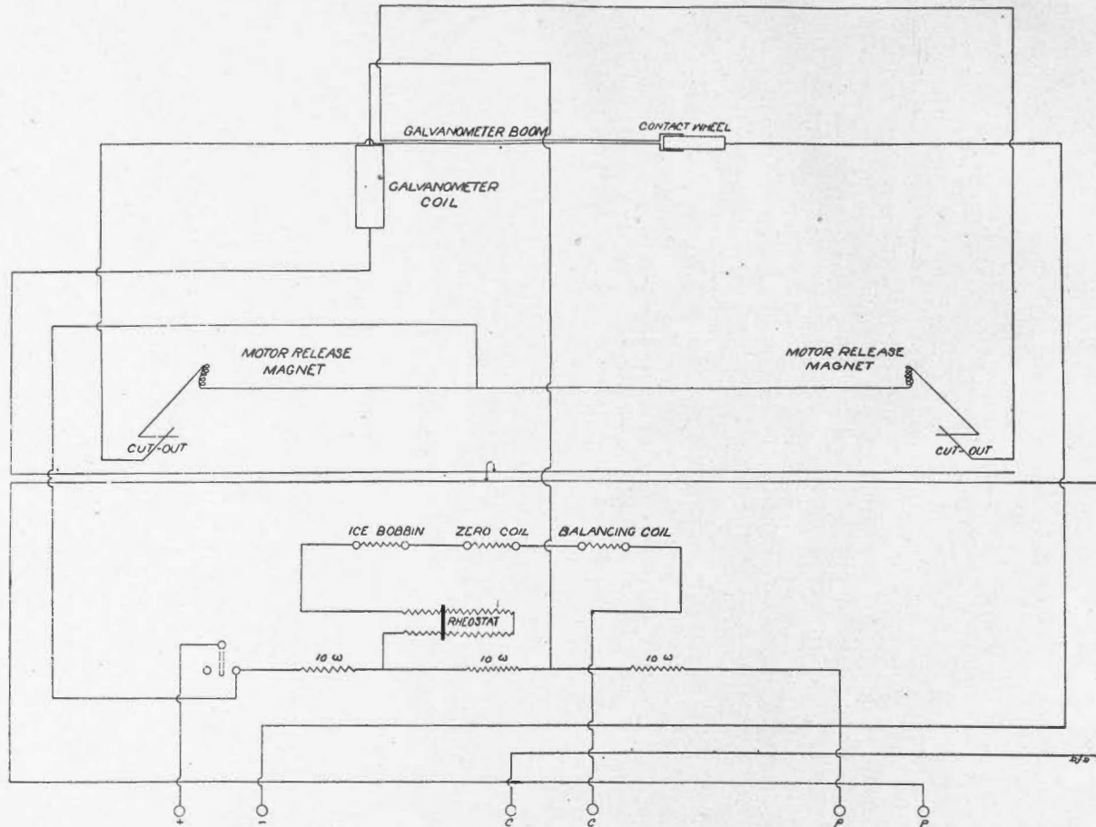
FIG. 2.—Electric Circuits of Callendar Recorder.
