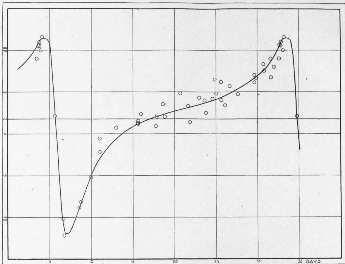
Fig. 8.—Velocity Curve of z Orionis.
