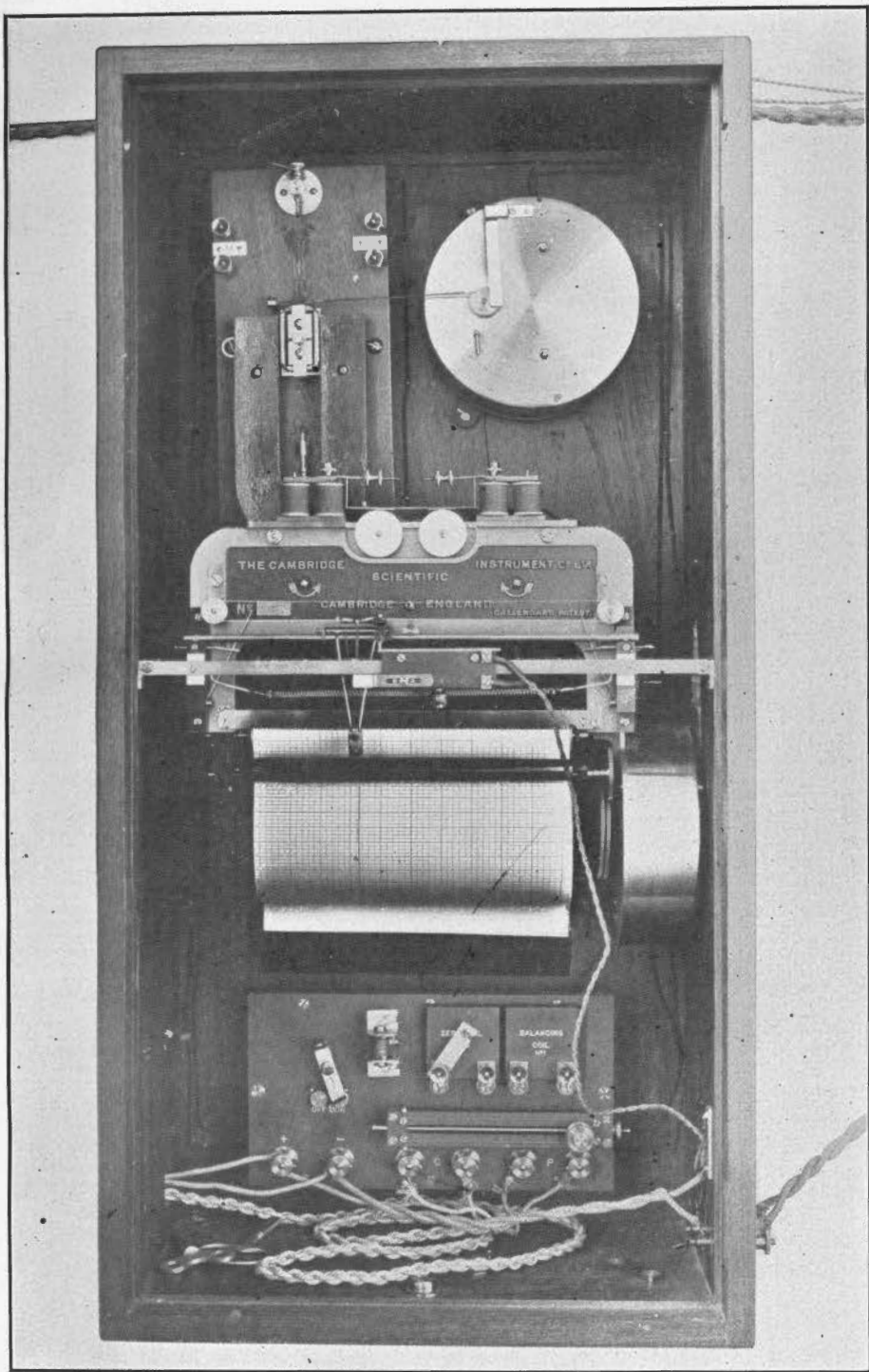
FIG. 1.—Calendar Electric Recorder.
