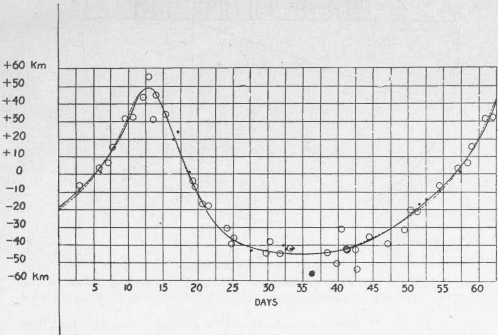
FIG. II.—Velocity Curve of a Draconis.
