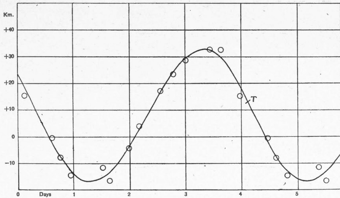
Radial Velocity Curve of \pi Arietis
