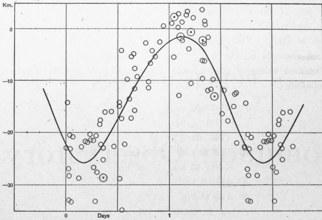
FIG. 1—Observations of \alpha Trianguli.
