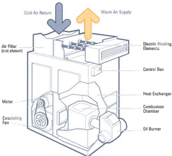
Figure 12: An oil-electric combination furnace
