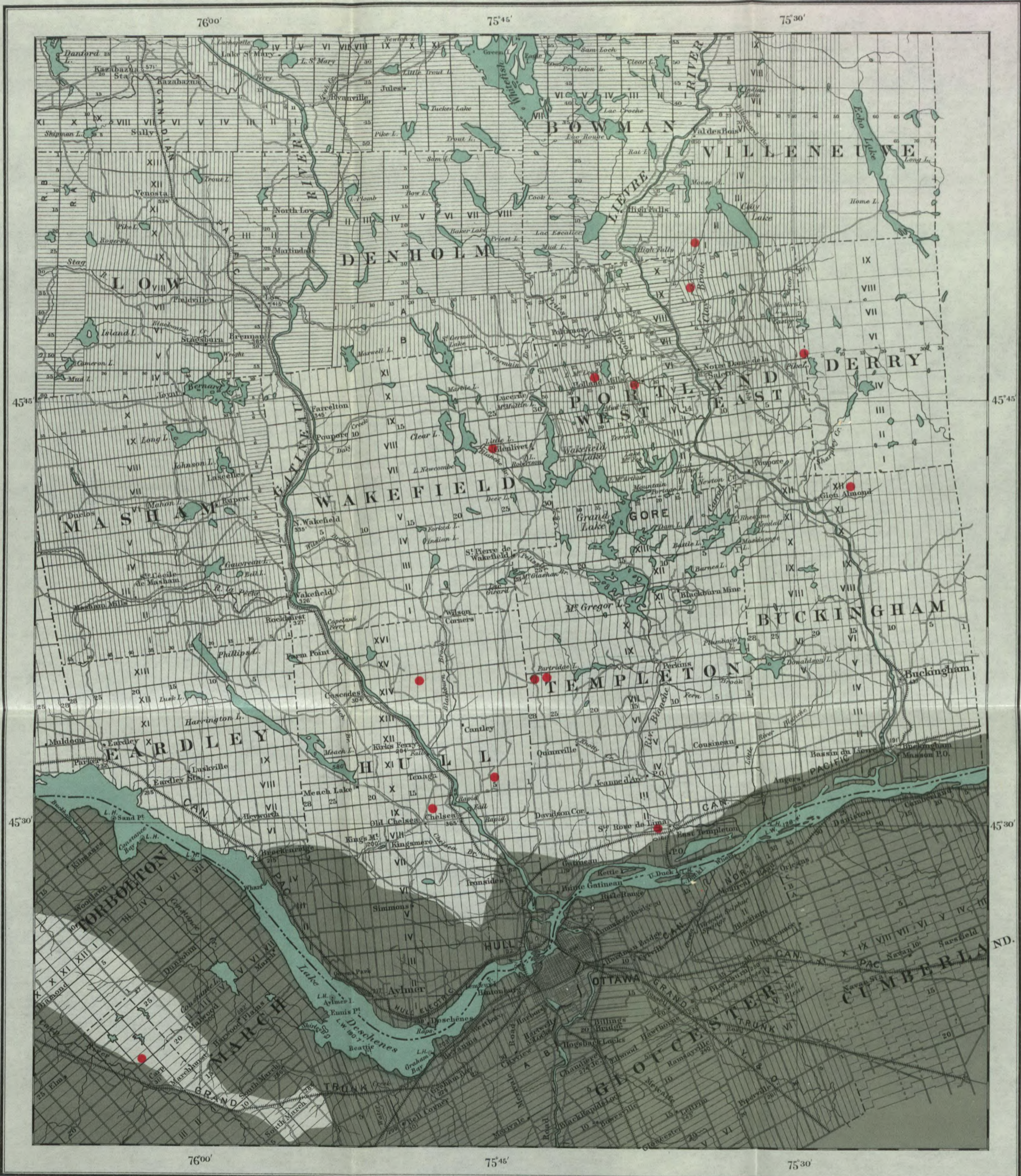
MAP SHOWING LOCATION OF THE PRINCIPAL FELDSPAR QUARRIES IN QUEBEC
