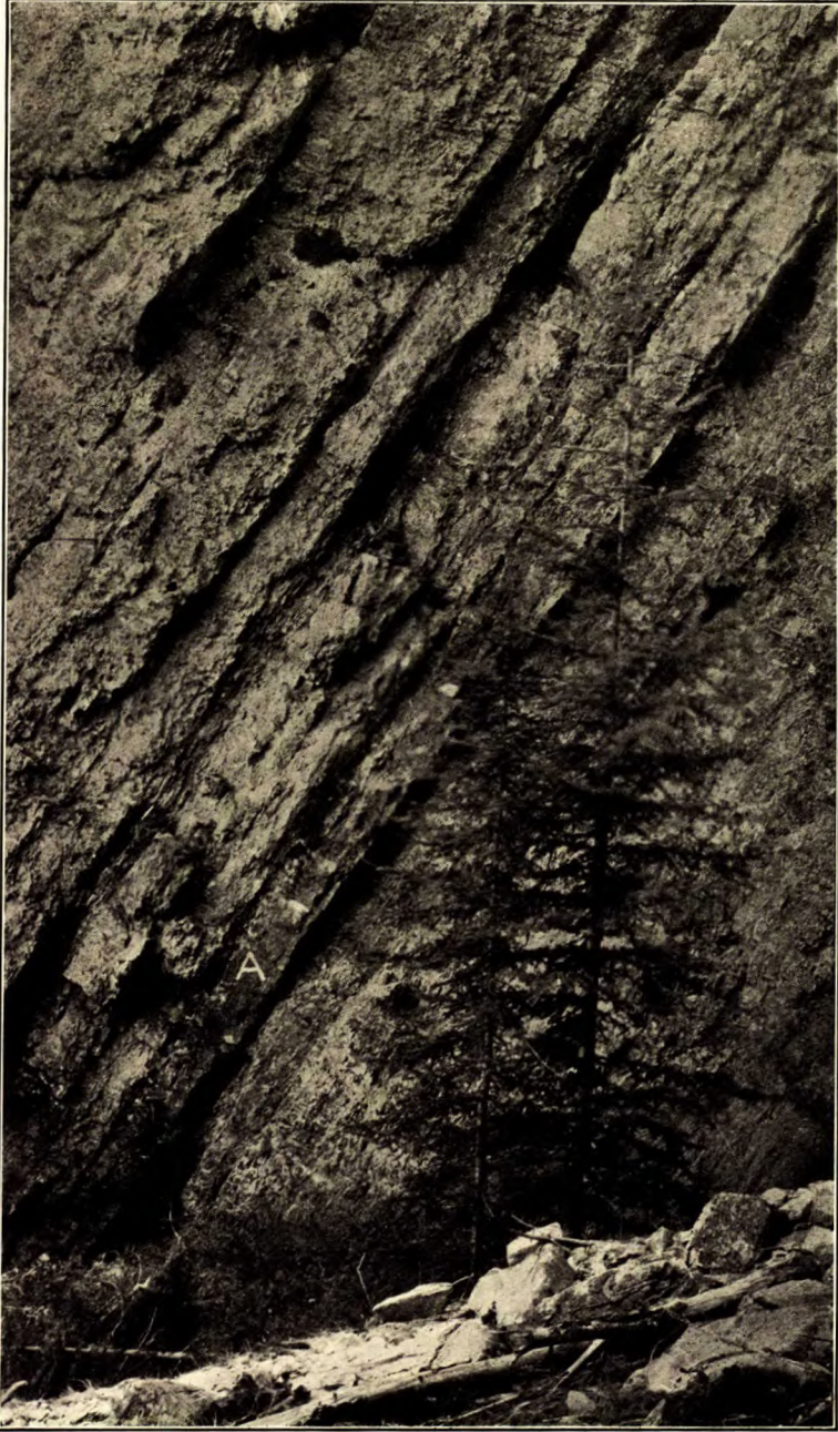
Tilted phosphoria beds at measured section in coulee on west side of Mount Norquay. The main bed (A) possesses the greatest thickness (2 feet) observed in the area examined, but is low in phosphoric acid.
