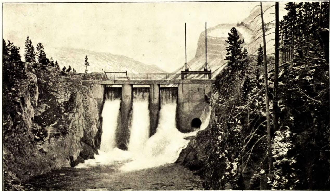
North end of Devil's canyon, showing dam at outlet, Lake Minnewanka. The beds shown are probably near the base of the Rocky Mountain quartzite, and the canyon, for the whole of its length (500 feet), is in this series. The course of the canyon is practically normal to the dip of the strata. The contact of Permian shales with the quartzite lies at the extreme end of the canyon; no trace of the Phosphoria formation was found in this fault-strip.
