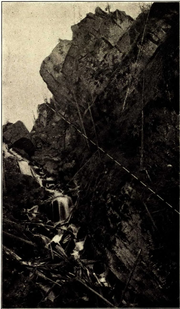
Tilted beds of the Phosphoria formation, Sundance canyon. The top massive ledge is a harsh chert-quartzite, representing the uppermost section of the Rocky Mountain quartzite. Directly below it follow the phosphatic beds. The position of the main phosphate bed is indicated by the dotted line.
