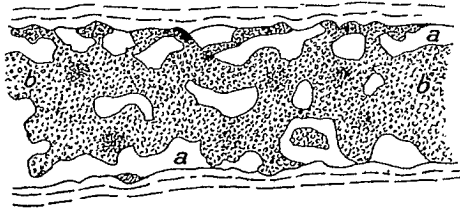
Fig. 1. Section of phosphate bed, showing nodular-massive occurrence of the phosphate ( b ) in a matrix of phosphatic quartzite ( a ), Sundance Canyon.
