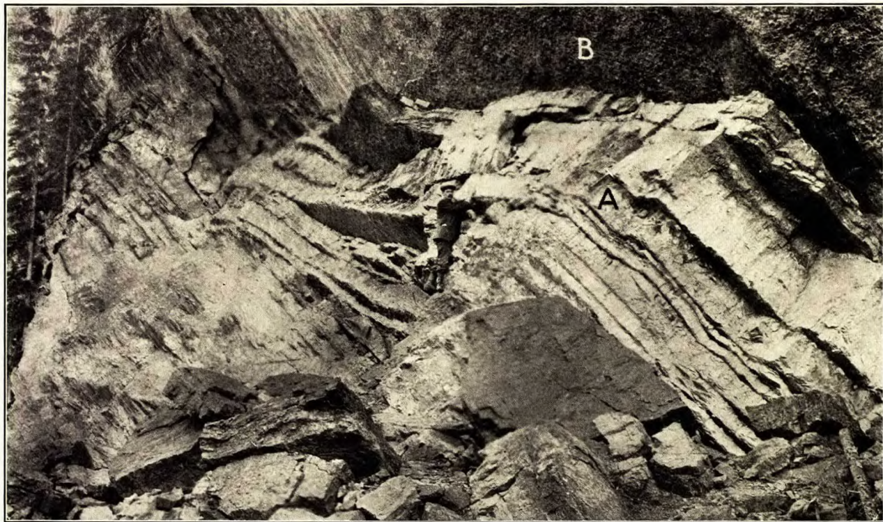
Phosphoria beds at measured section, Sundance canyon. The main bed (A) lies some 6 feet below the chert-quartzite capping (B). Practically all the beds shown yielded some trace of phosphoric acid.
