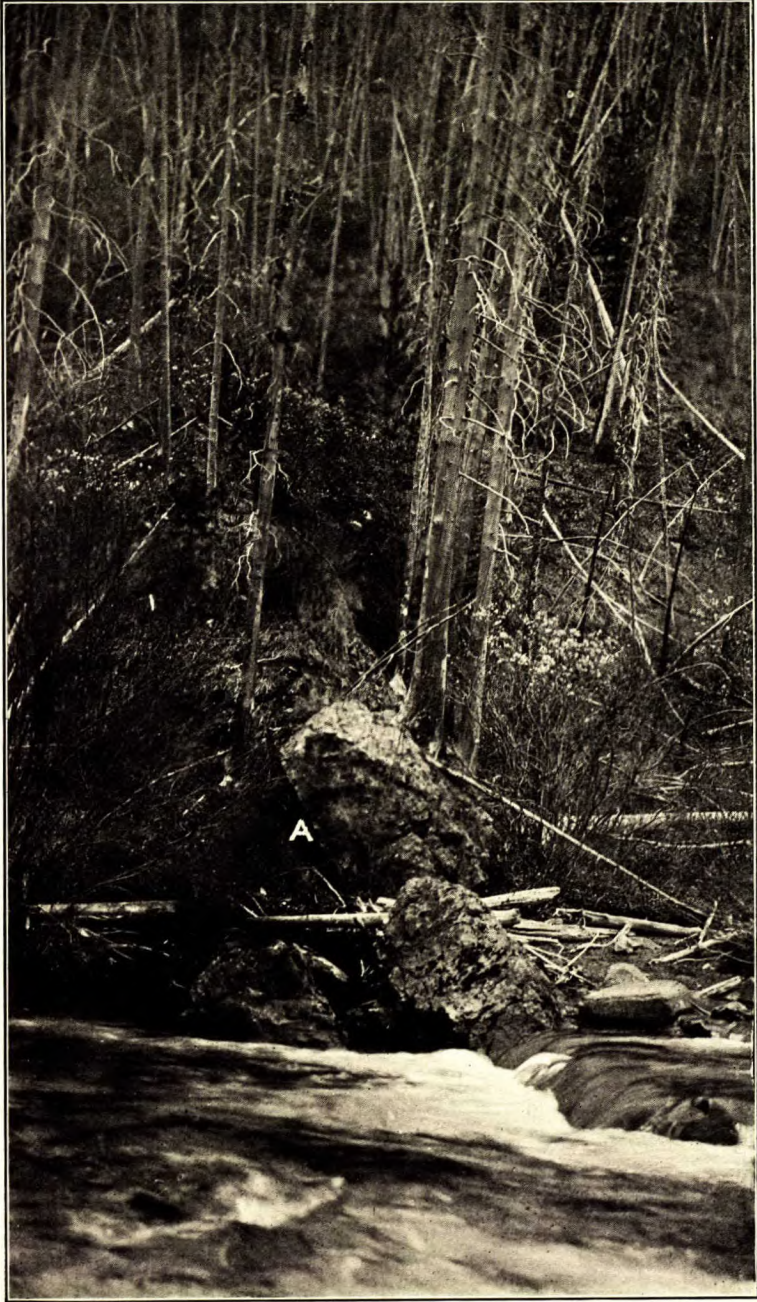
Outcrop of main phosphate bed (A) between quartzite ledges on right bank of Forty-mile creek.
