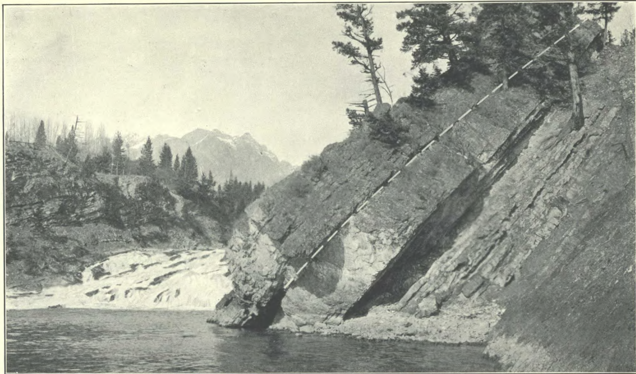
Exposure of phosphoria beds at Bow Spray falls, Bow river. The main phosphate bed occupies the position shown by the dotted line. The right bank of the river and the river bed itself are formed of Permian shales.
