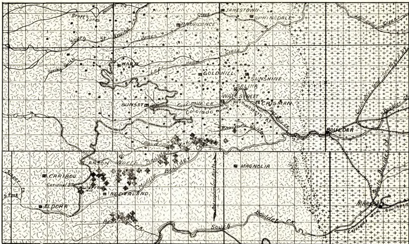
GEOLOGICAL SKETCH MAP, BOULDER COUNTY TUNGSTEN AREA.
