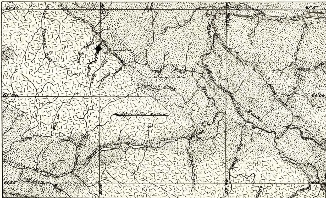
GEOLOGICAL SKETCH MAP PART OF CAPE BRETON ISLAND TUNGSTEN AREA
