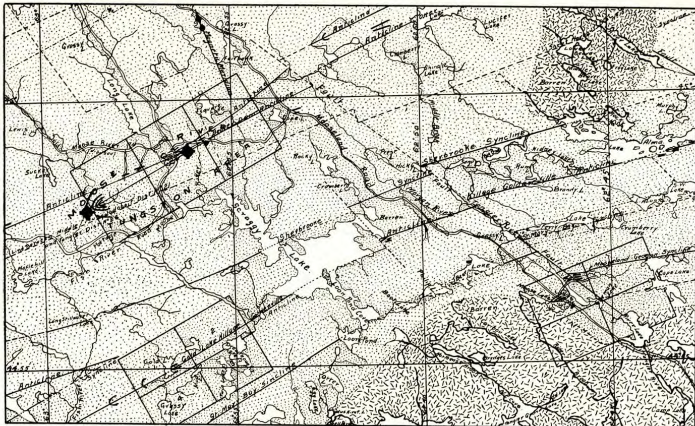
GEOLOGICAL SKETCH MAP MOOSE RIVER TUNGSTEN AREA
