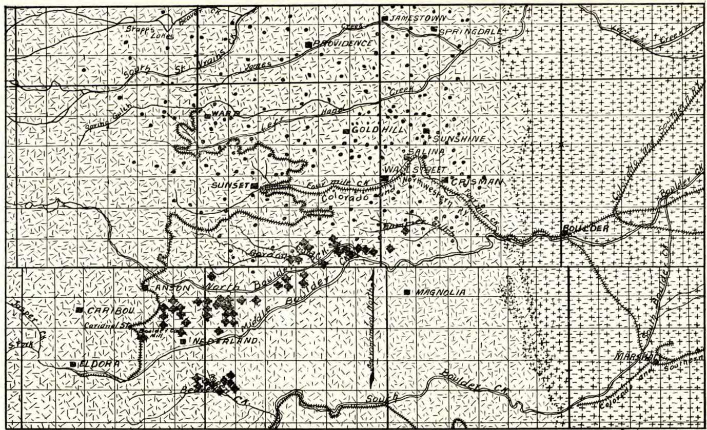
GEOLOGICAL SKETCH MAP, BOULDER COUNTY TUNGSTEN AREA.
