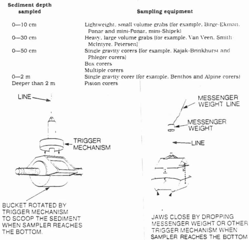
FIGURE 2. Grab samplers with their essential parts (Hudrock and Mackinlay, 1991)
