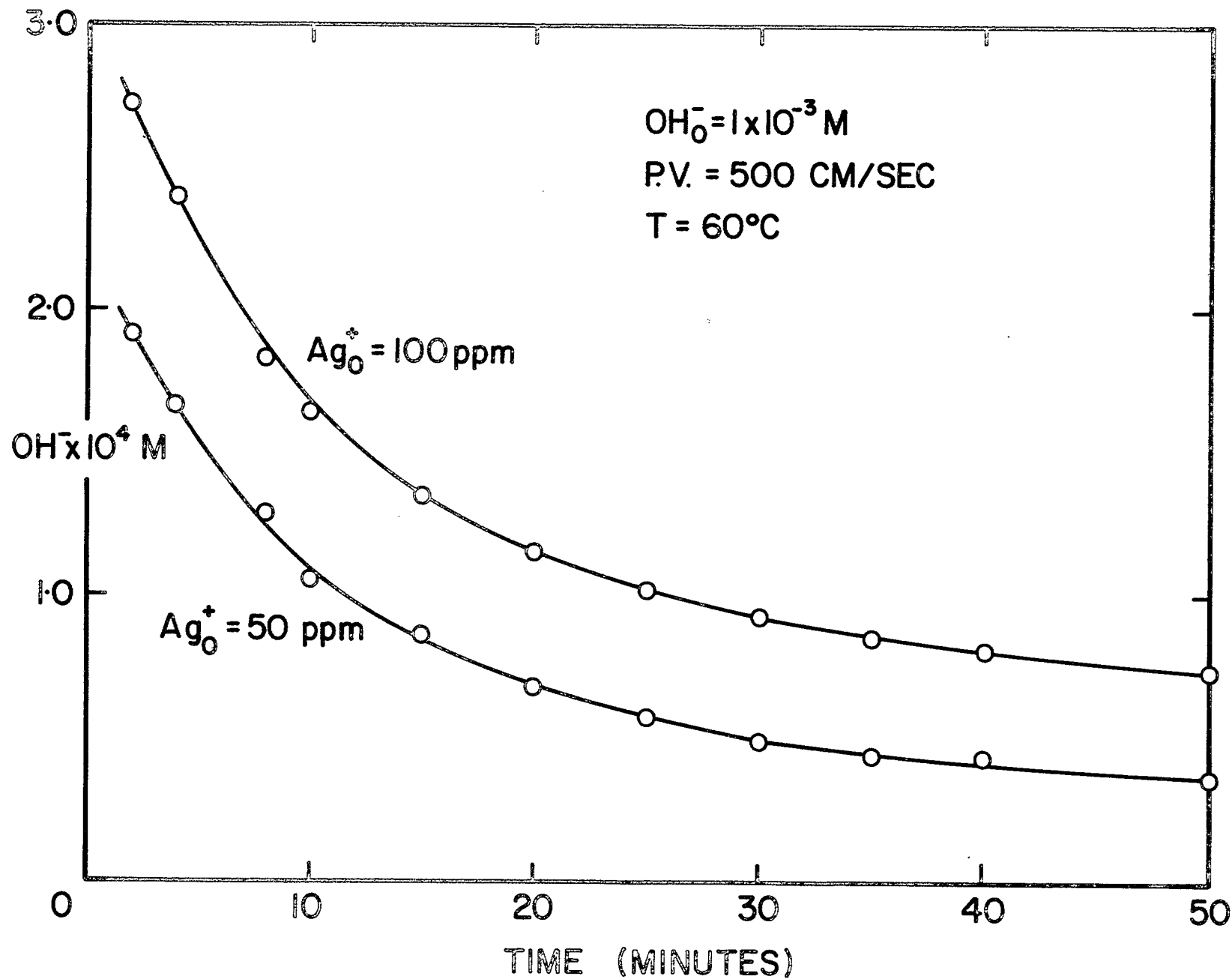
Figure 5. Plot showing the decrease in OH - with time for silver cementation on aluminum.
