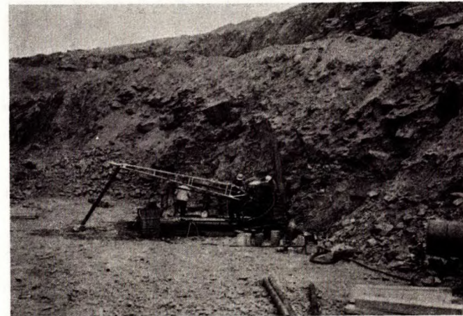
4. Drilling the Anchor Holes.
