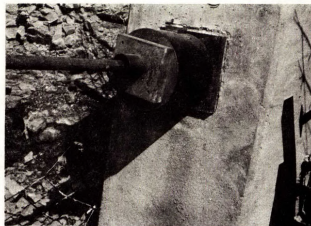
42. Stressteel Anchor and Load Cell.
