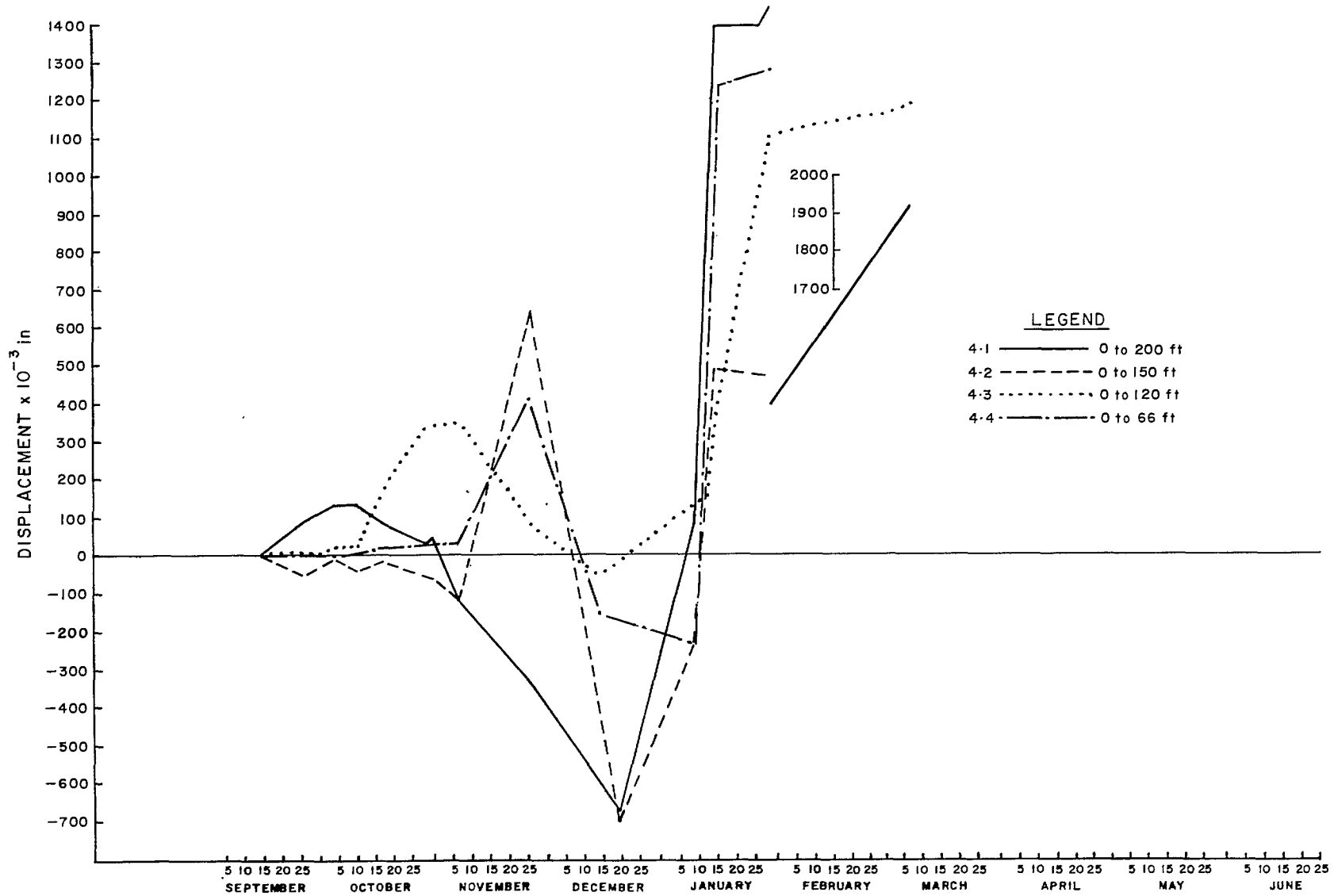
Figure 23. Extensometer No. 4.
