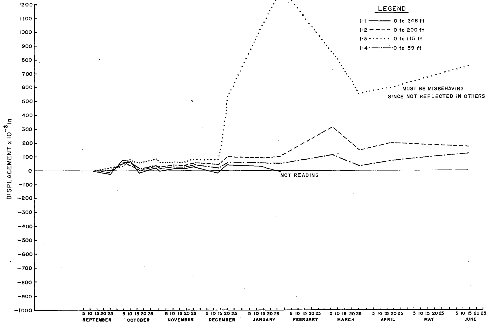
Figure 20. Extensometer No. 1.
