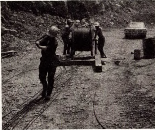
9. Cable Anchor Assembly - 12 Strand Cable Assembled on Site from Individual Strands.
