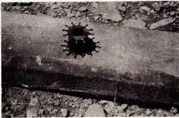
11. Cable Anchor Assembly- Strand Spacer.
