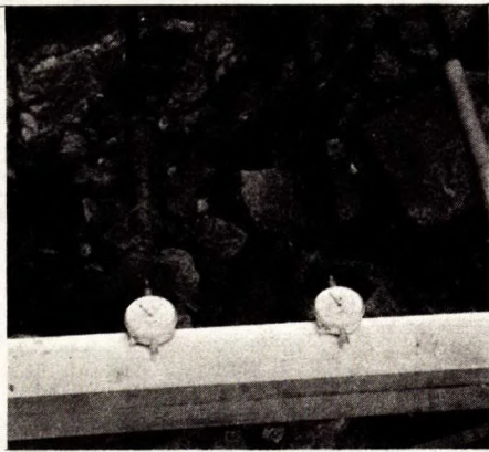
35. Dial Gauges Probing Surface Studs.
