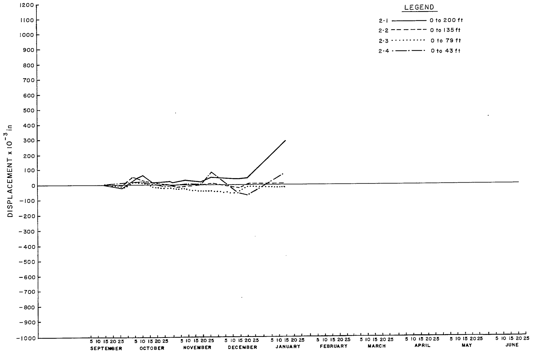
Figure 21. Extensometer No. 2.
