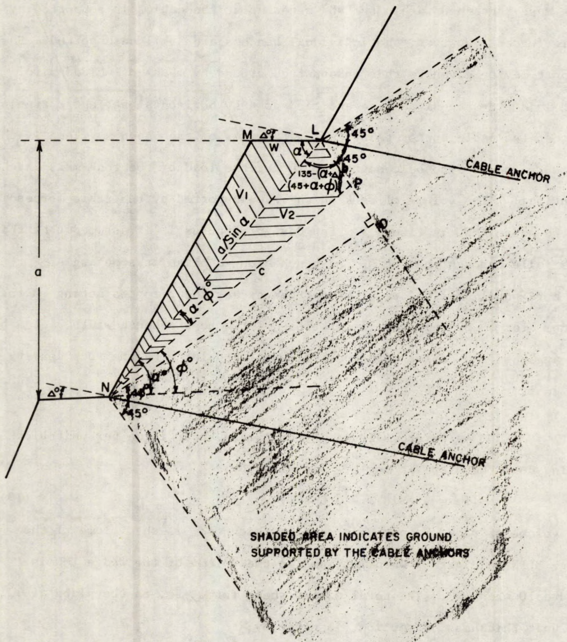
Figure 9. Rock volume involved in bench stability analysis, \phi < \alpha .
