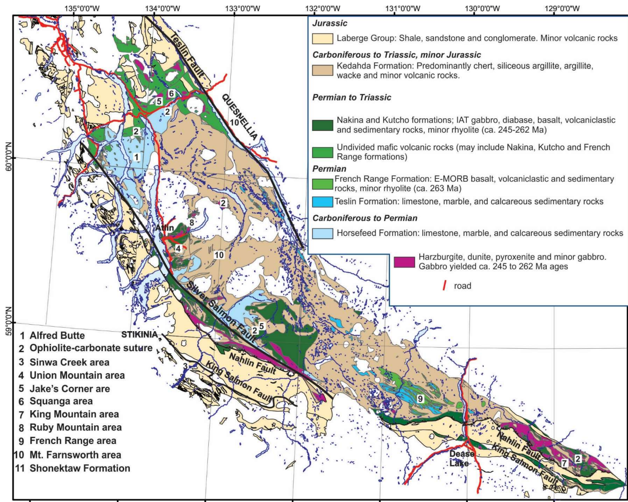
Figure 2 Simplified geology of the northern Cache Creek terrane showing the distribution of various tectono-stratigraphic units (simplified from Massey et al. 2005 and Colpron 2015)
