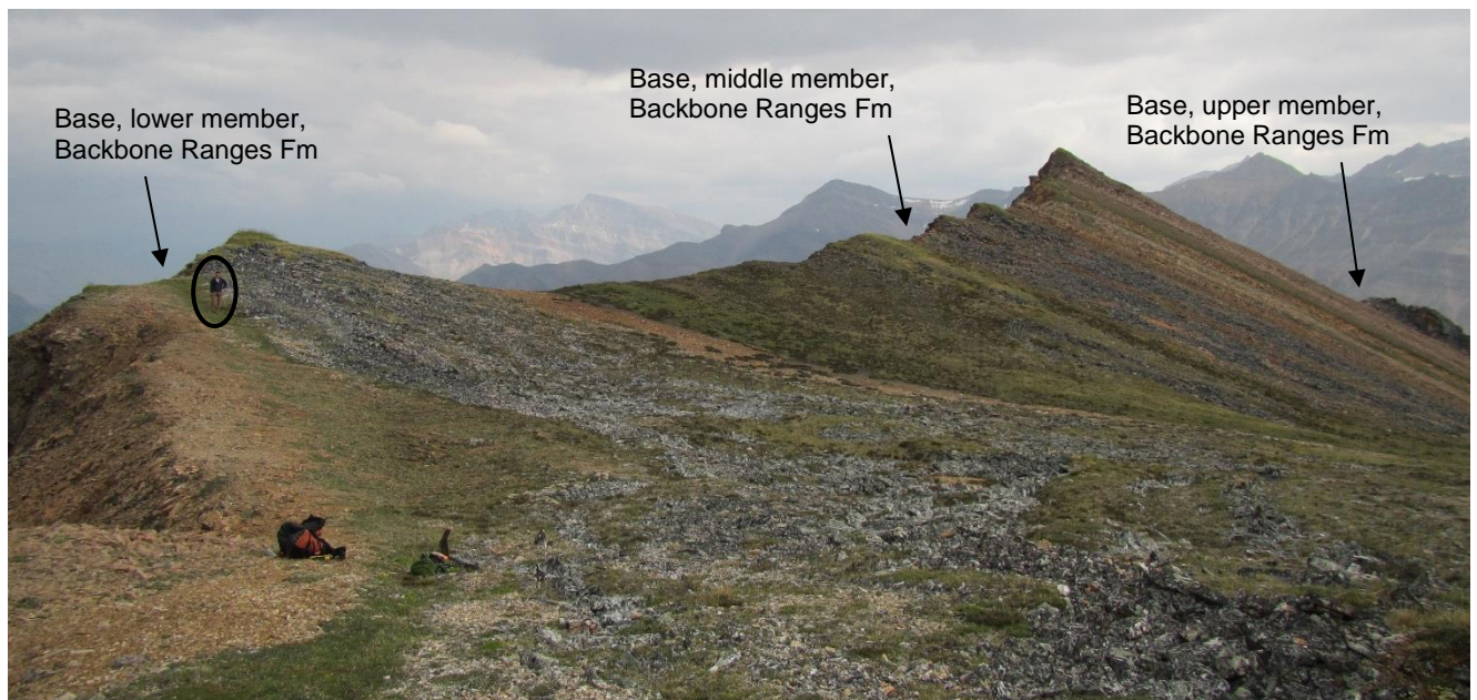
Figure 5: Overview of measured section MWB17B. Orange-weathering strata at left belong to the “Sheepbed carbonate”. Basal contacts of members of Backbone Ranges Formations are marked by arrows (labelled). Person for scale (circled at left) . See Figure 2 for location.
