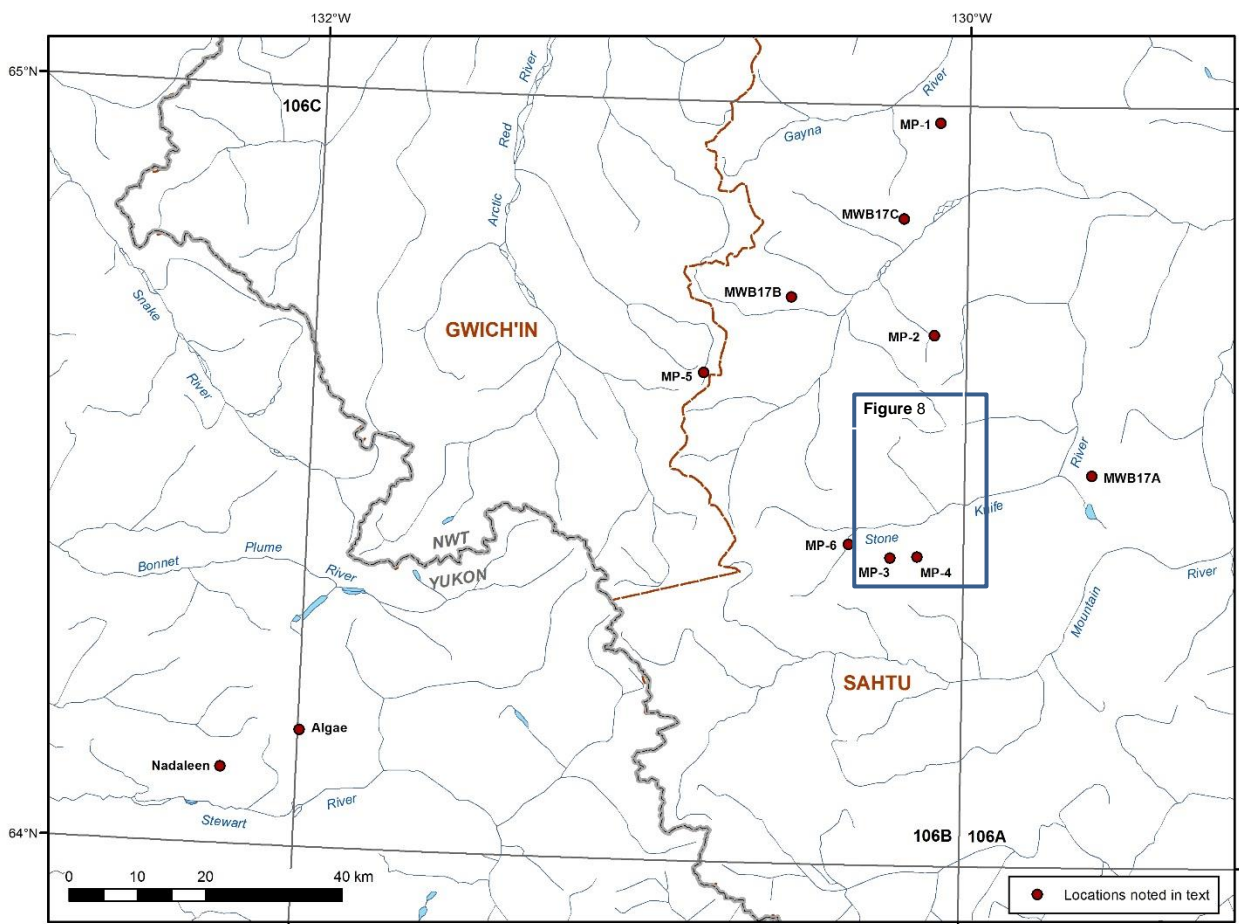
Figure 2: Detailed location map of 2017 study area (NTS 106-B). Blue inset box shows general area of mineral deposit studies; for detailed map of visited mineral localities, see Figure 8.
