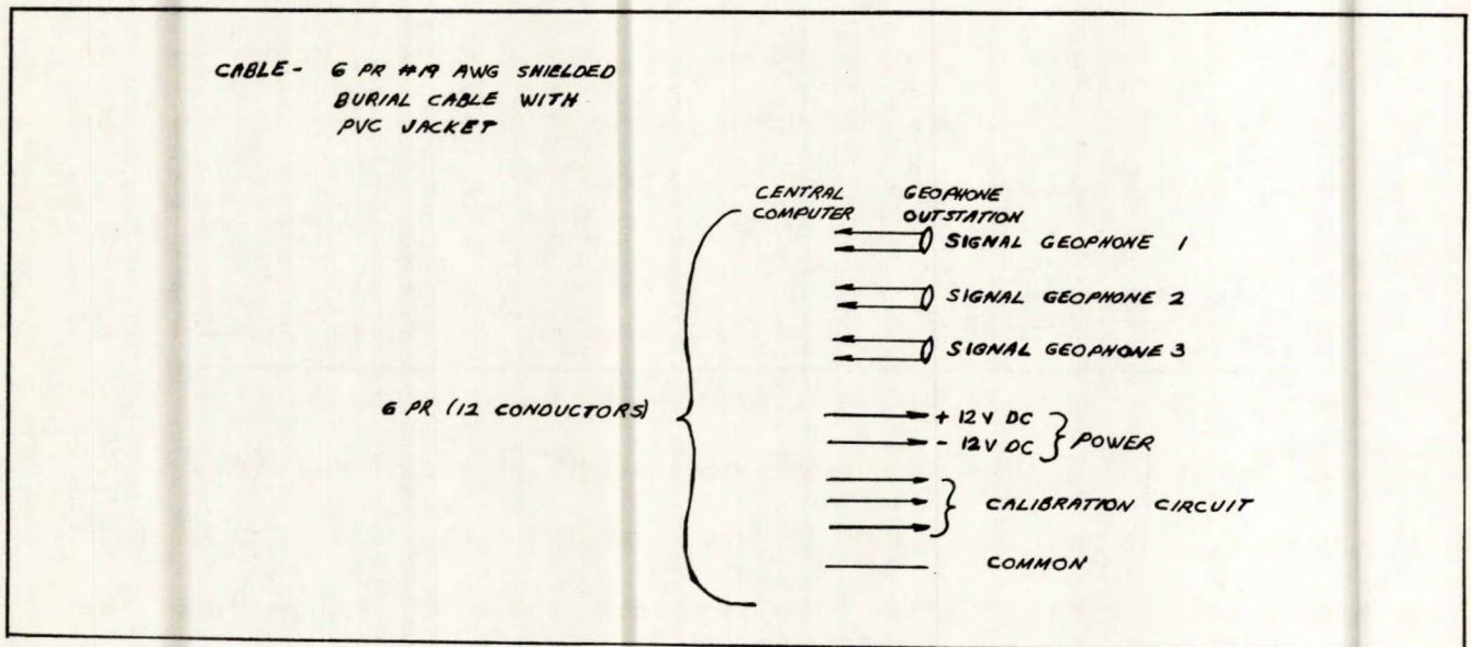
Fig. 6 - Cable assignments.
