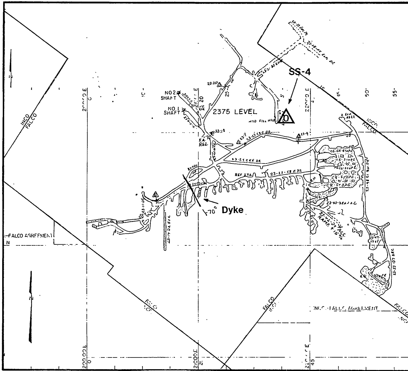
Fig. 2 - Plan of 2375 level showing sensor location.
