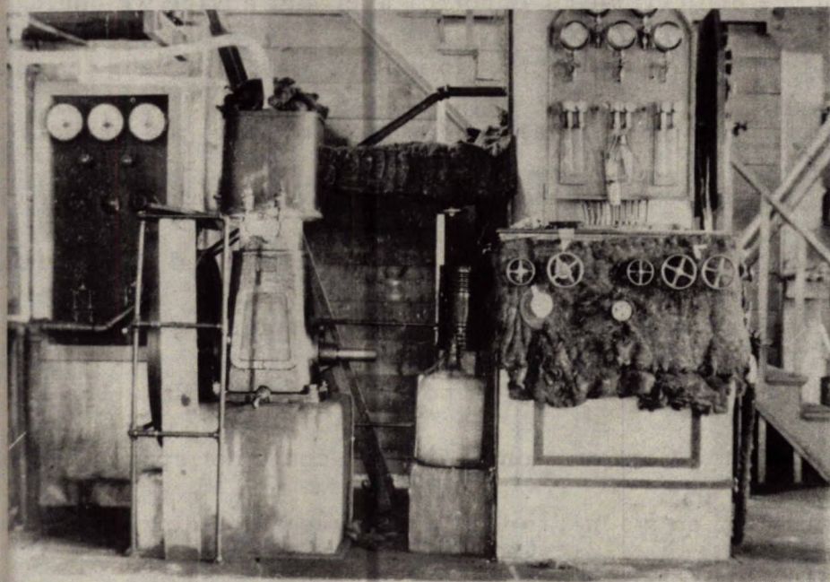
Figure 1 - The only photograph taken of the Hamilton machinery. The machine shown at left centre is the well-drilling apparatus.
