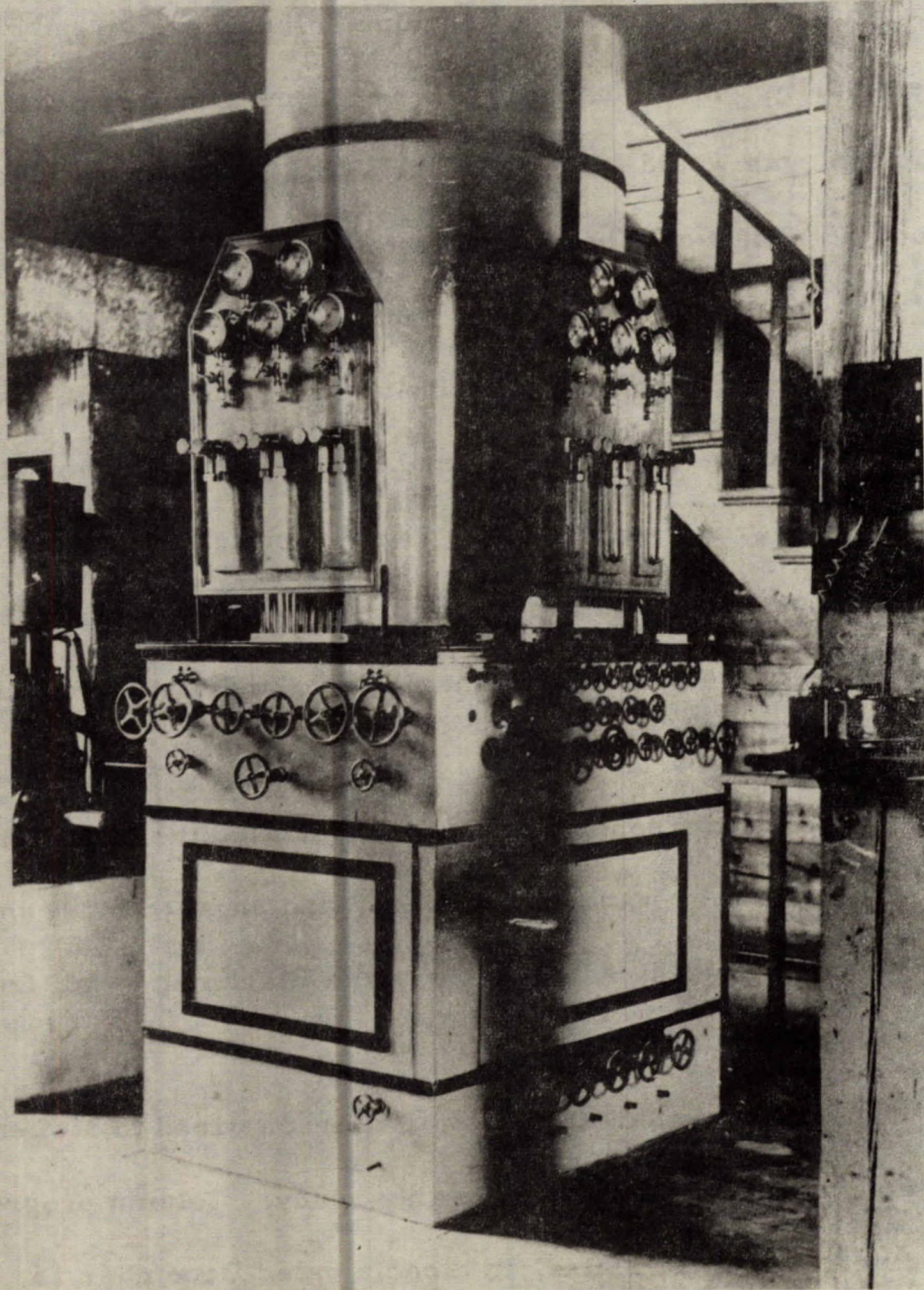
Figure 4 - The two-stage liquefier column used at Calgary. The valves and gauges on the left were used during the first stage and those on the right for producing the final product. The galvanometer on the post was used to control the temperatures at various places in the column by means of thermocouples.
