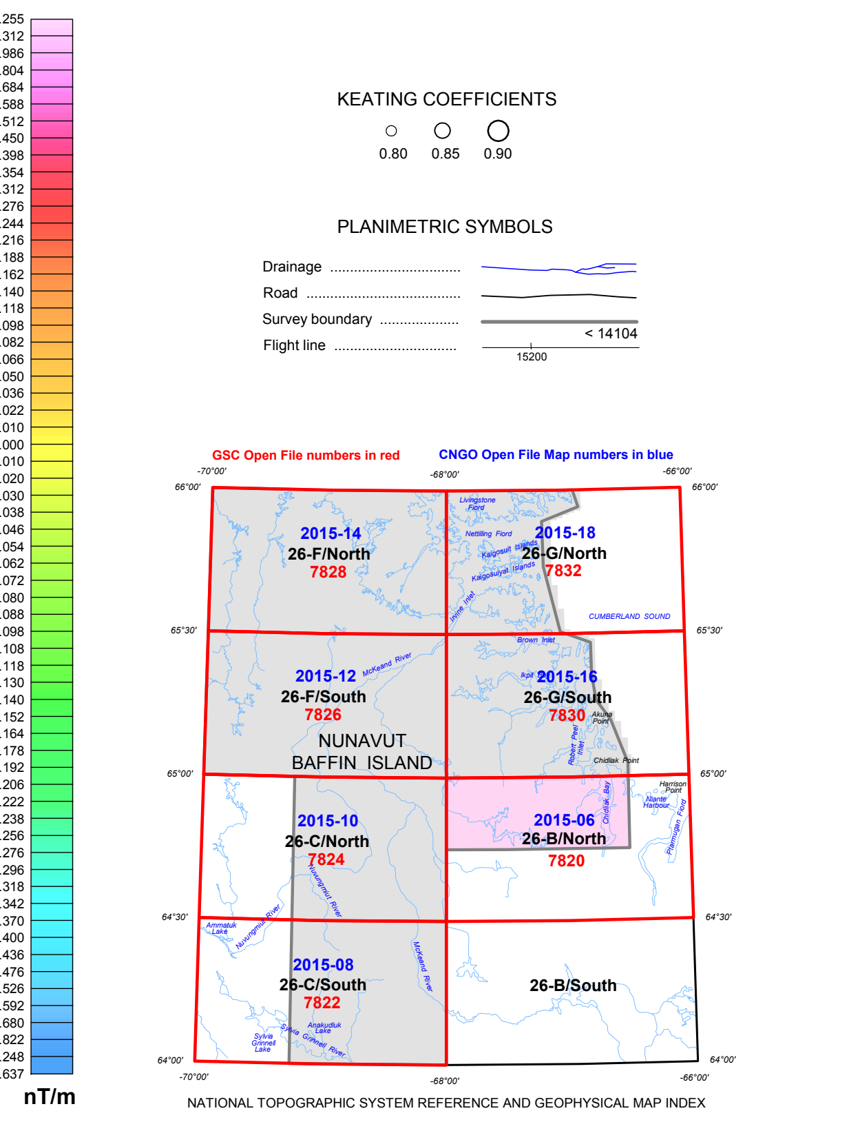
AEROMAGNETIC SURVEY OF THE MCKEAND RIVER AREA
