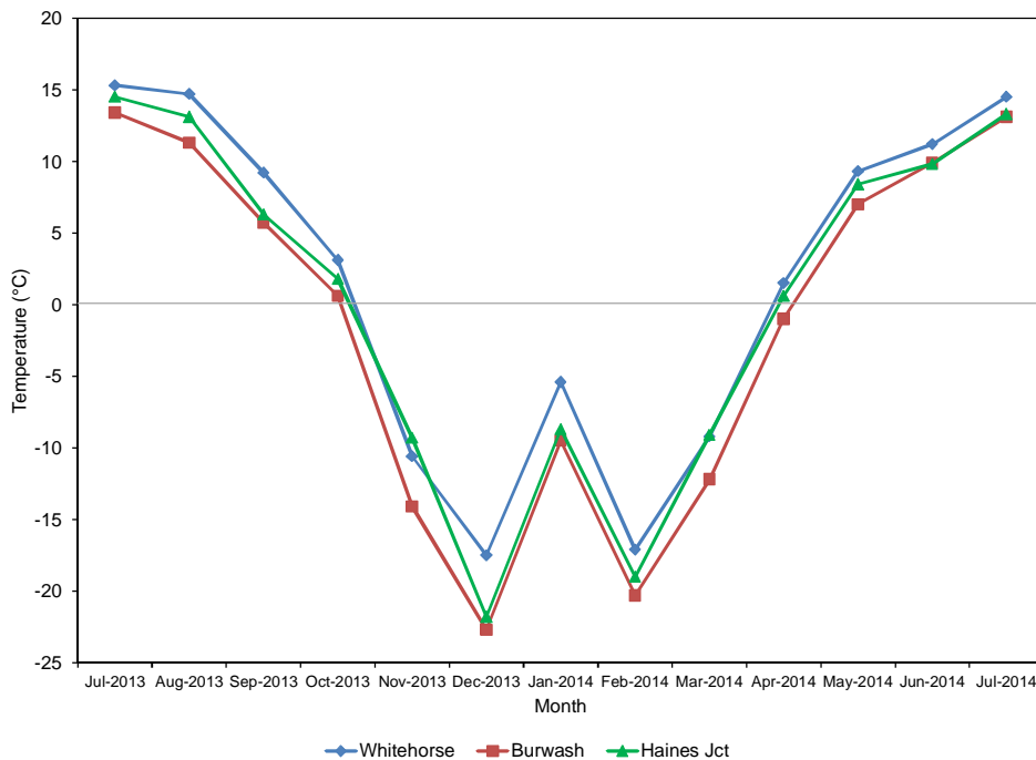
Figure 2. Mean monthly air temperatures July 2013 to July 2014 for Environment Canada stations at Whitehorse, Haines Junction and Burwash Landing (data from Environment Canada, 2015).
