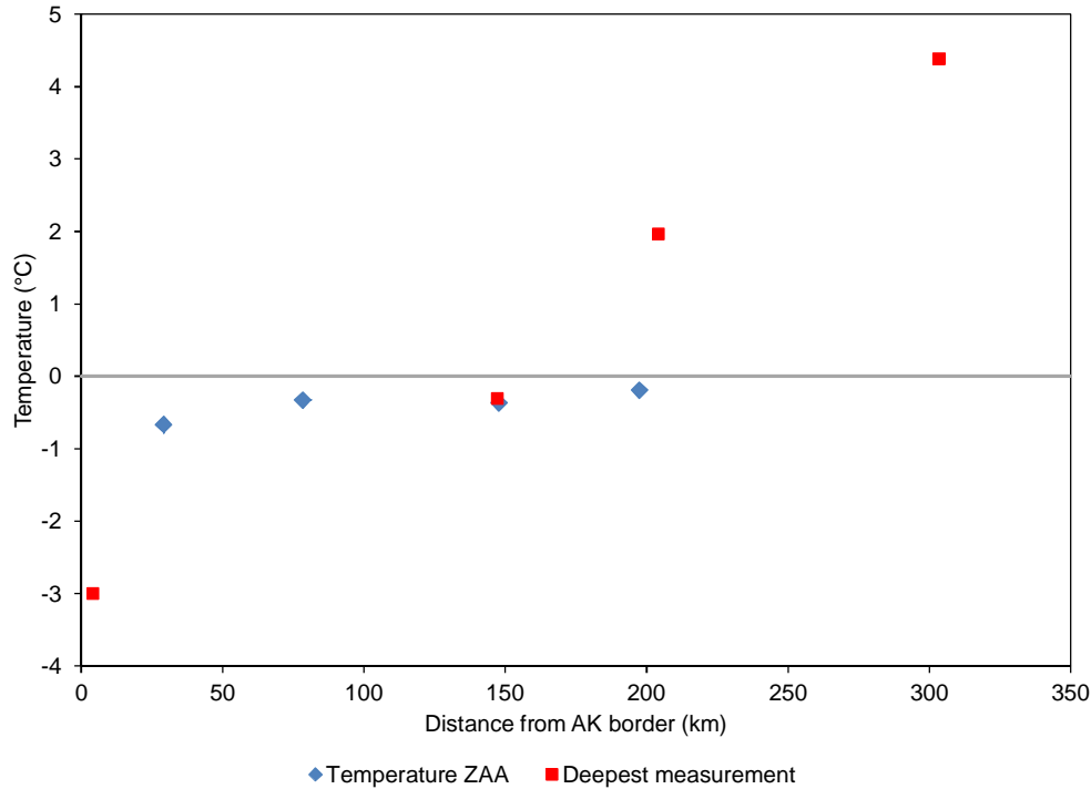
Figure 5. Mean ground temperature for 2013-14 along the corridor (distance given from Alaska border). Mean temperature is determined for the depth of zero annual amplitude (ZAA) or deepest measurement depth.
