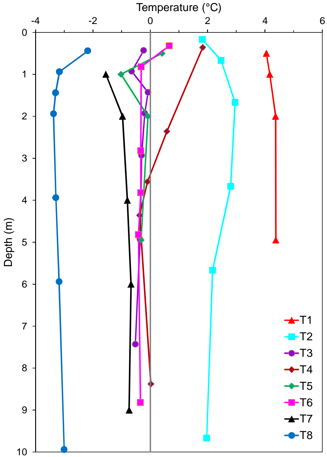
Figure 4. Annual mean ground temperature profiles for 2013-14 (July 15 2013 to July 14 2014).
