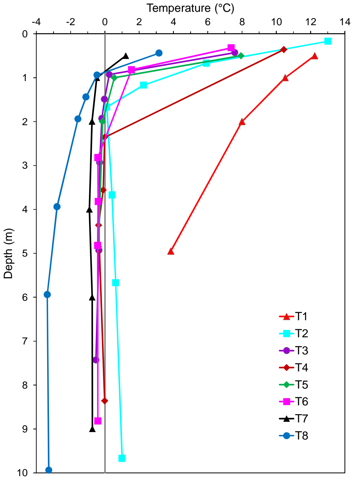
Figure 3. Ground temperatures measured during sites visits between July 30 and August 1, 2014.
