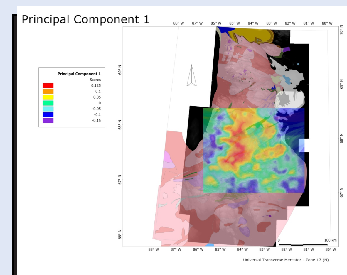
Figure 5. Map showing the first component plotted over the regional geology and digital elevation model for the area. Positive scores are associated with the upper elevations of the digital elevation model representing a relative increase in Al-Ga-K-V-Mg-Pb-Co-Th-Mn-Fe-Cr-Rb. This combination of elements is interpreted to represent the concentration of mineralogies associated with the homogenization of regional bedrock lithologies resulting from glaciation.
