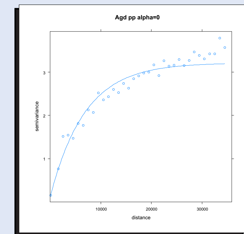
Figure 8. Fitted semi-variogram for posterior probability of lithology Agd.
