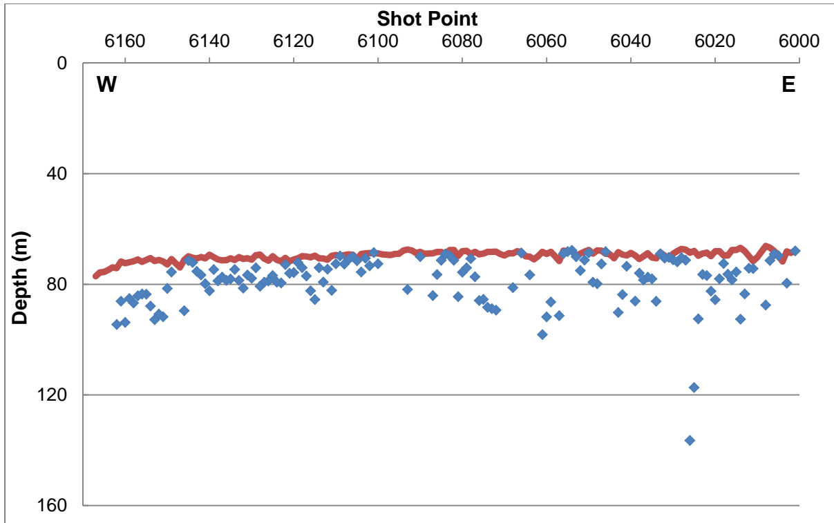
Figure 10I. Results of refraction analysis along Line-6 of Expedition ARA04C showing depth of first refraction in meter below sea-surface (blue diamonds) and seafloor determined from MCS data (dark red line). Shot-numbers increase from E to W.
