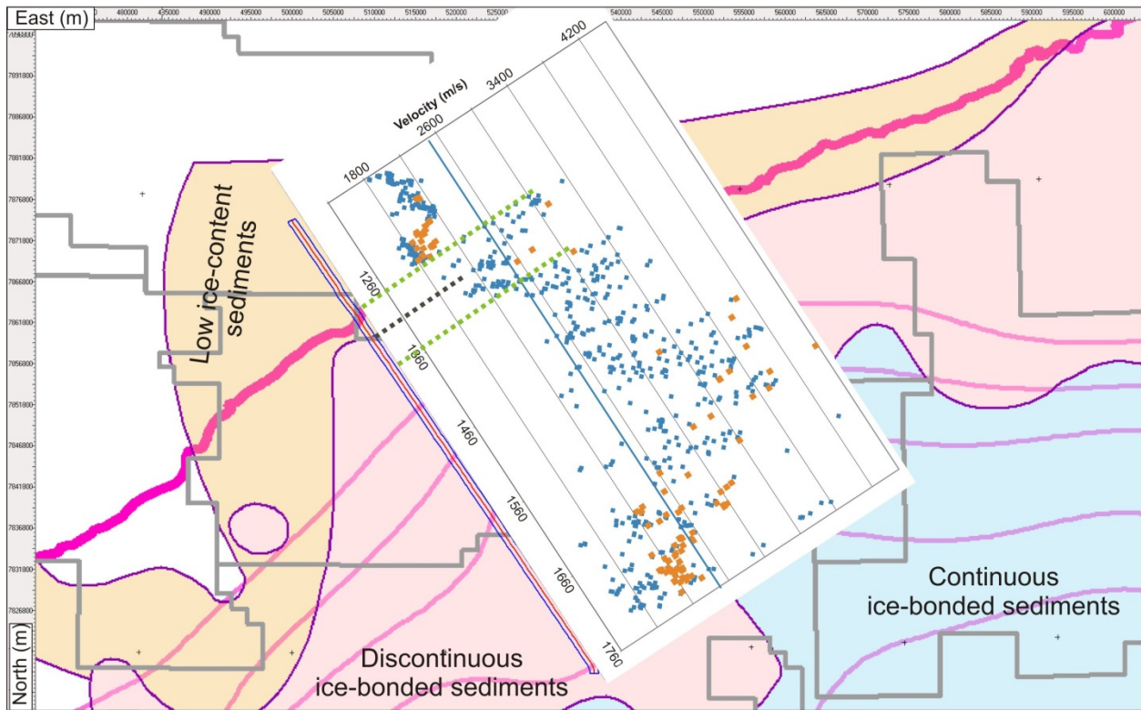
Figure 11a. Map of Pullan et al. (1987) with distribution of ice-bearing sediments and location of Line-1 of Expedition ARA04C. Superimposed are the velocity values (as Figure 10a). The suggested boundary between discontinuous (pink) and low-ice content (yellow) sediments is bracketed by the new velocity results along this line around shot point 1310.
