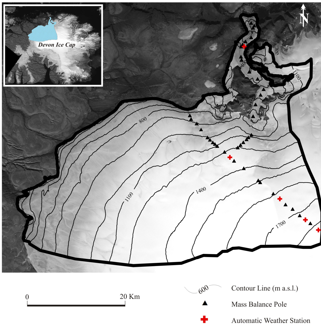
Figure 2. Location of mass balance pole network and automatic weather stations in the Northwest sector of the Devon Ice Cap. Background is a LandSat ETM + satellite image acquired in July, 2000. Inset in top left indicates the location of the Northwest sector (shaded blue) within the ice cap.
