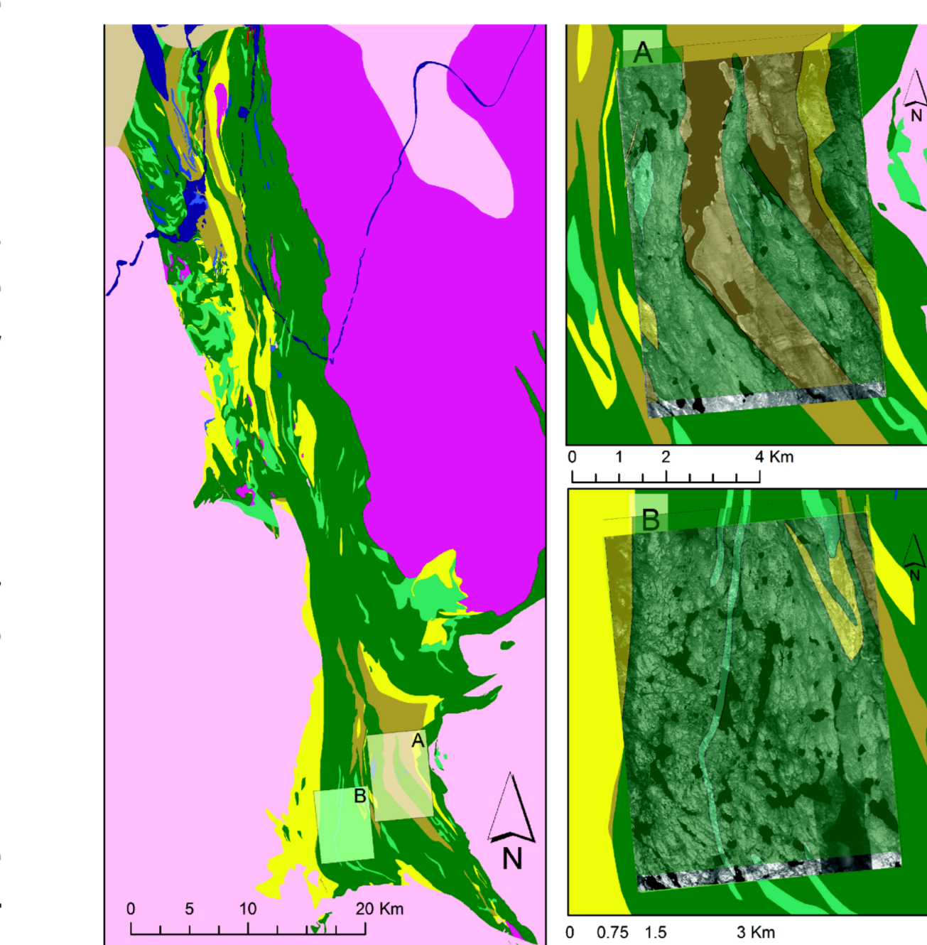
Fig 2: Simplified geology map showing location of study regions A and B. Region A contains the Boston deposit; region B is located to the south west of the Boston deposit, and contains no known deposits (modified from Stuble, 2005).
