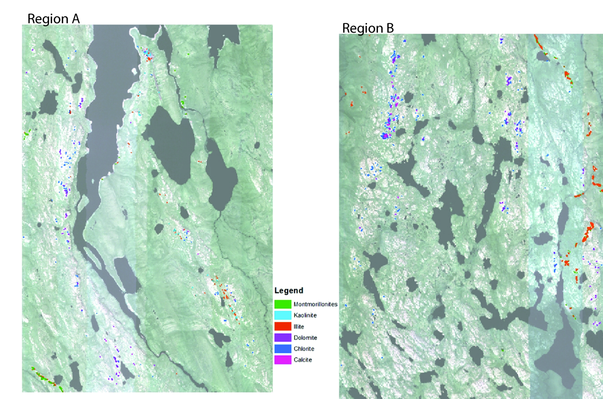
Fig 12. (above left) and Fig 13. (above right): Hydrothermal alteration mineral distribution maps overlaid on airborne RGB data used in the initial analysis for the two study regions A and B.
