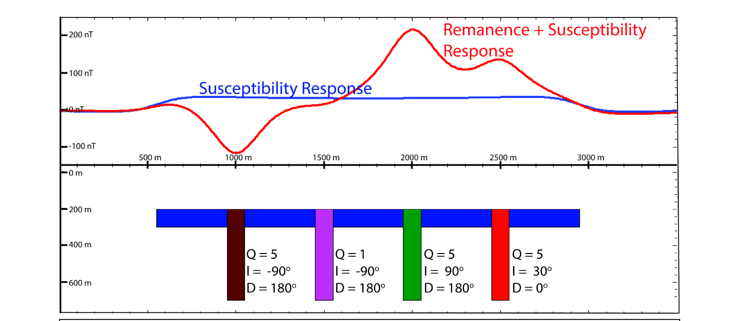
Figure 2: Consider a simple model where a near surface horizontal sheet is intruded by a series of tabular bodies (dikes). If all of the five bodies have exactly the same susceptibility then the observed magnetic anomaly pattern would show the signal for a simple tabular body. If the tabular bodies have a strong remanent magnetisation signal, as diabase dikes often do, then the actual observed magnetic anomaly pattern would be very different from the simple single tabular body anomaly.
