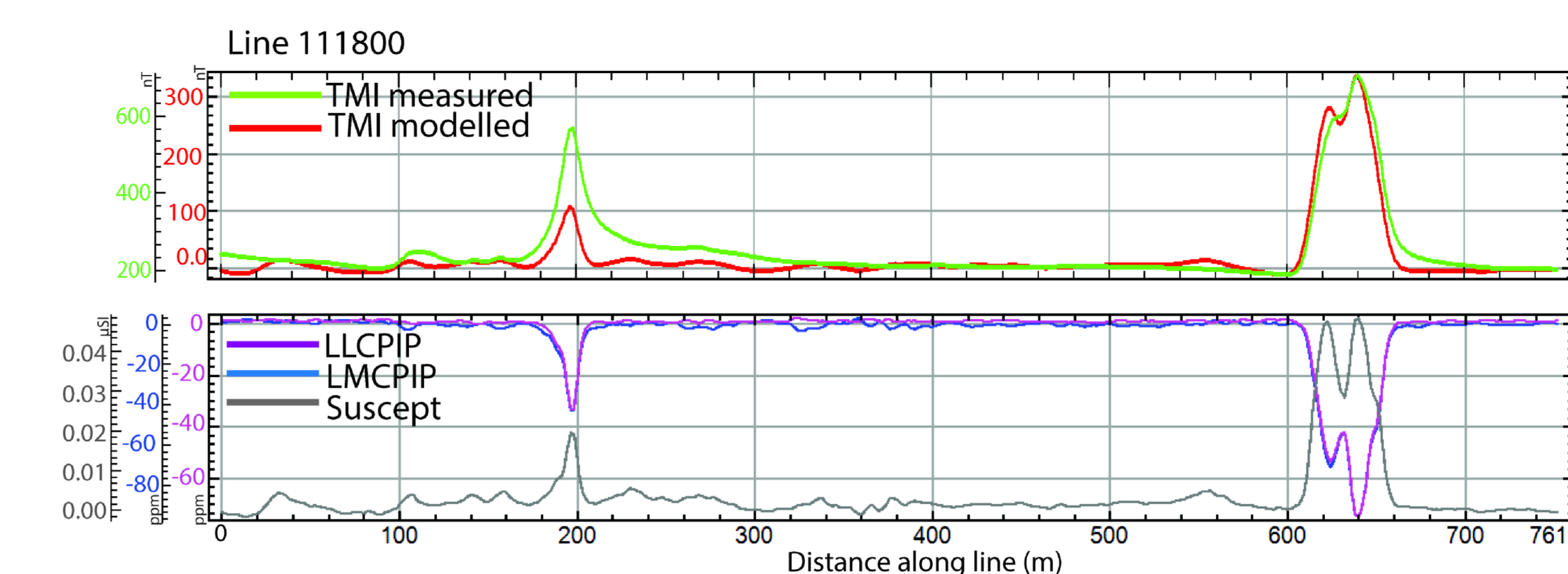
Figure 5: Profile along line 111800. There is good correlation between measured and modelled magnetic anomalies (Top) where susceptibility is successfully recovered from low (LLCPIP) and medium (LMCIPI) coplanar in-phase data (Bottom).
