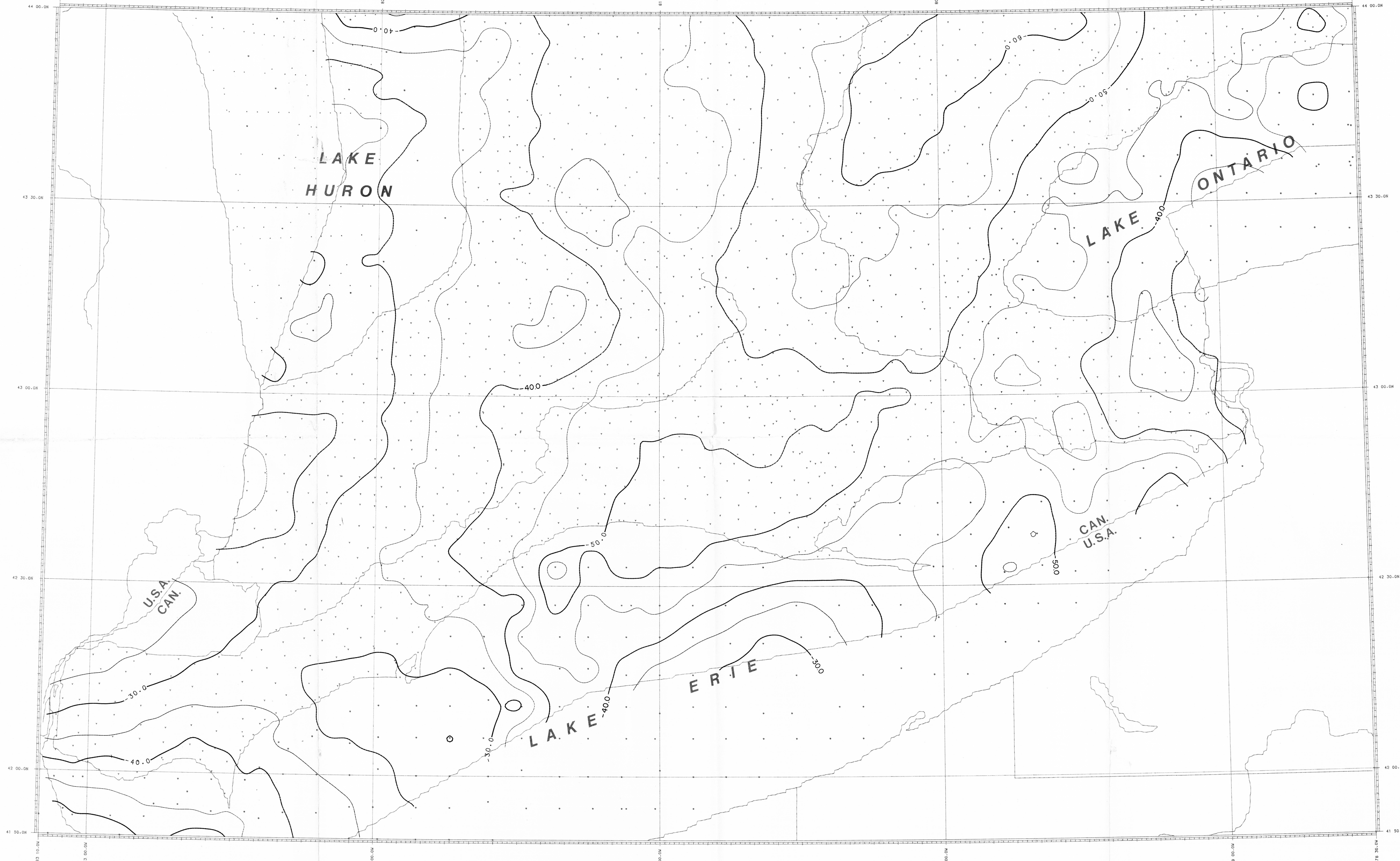
-BOUGUER ANOMALY MAP- Scale 1:500,000 Projection U.T.M.
