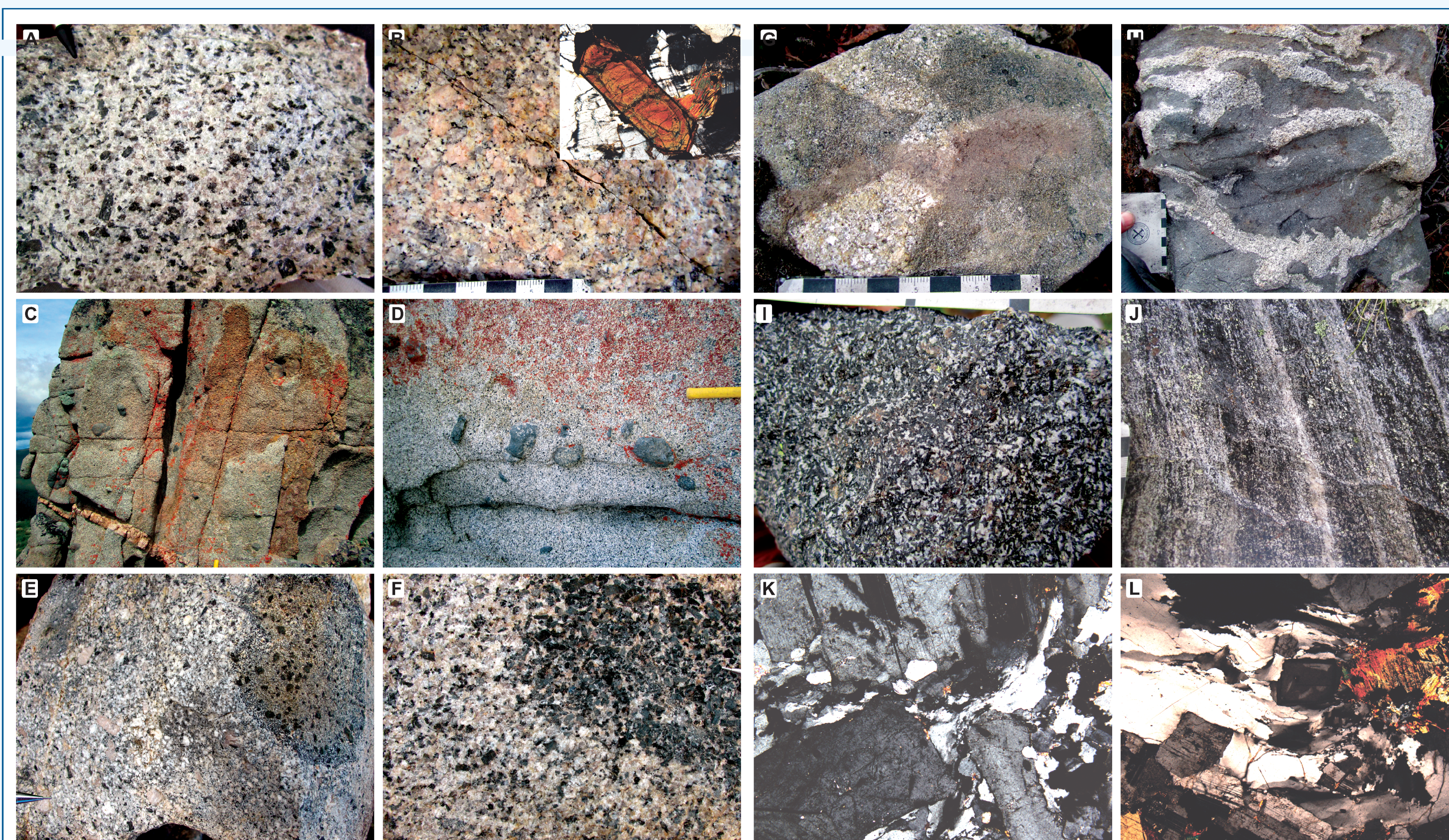
Representative photographs of Whitehorse Plutonic Suite in the Dawson Range area. A. Dawson Range phase hornblende-biotite granodiorite with characteristic blocky hornblende. B. Coffee phase biotite syenogranite (Isaac Hayes pluton), inset: large allanite crystals are common in this phase. C. Characteristically abundant cognate hornblende diorite and gabbro inclusions in the Dawson Range phase. D. Train of diorite inclusions derived from a co-magmatic diorite dyke. E. Hornblende porphyritic diorite enclave in K-feldspar porphyritic, biotite-hornblende Dawson Range monzogranite. F. Hornblende diorite enclave in Dawson Range phase hornblende-biotite granodiorite. G. Dawson Range phase monzogranite dyke cuts hornblende quartz diorite. H. Pillowed diorite in Dawson Range phase monzogranite indicate coeval mafic and felsic magmatism. I. Hornblende-biotite diorite from a discrete diorite stock. J. Interlayered strongly foliated hornblende-plagioclase cumulate may form part of the basal Dawson Range suite. K, L. Photomicrographs of deformation fabrics in the Dawson Range phase granodiorite. Deformation is localized in quartz, locally resulting in development of quartz ribbons, and along grain boundaries, where plagioclase subgrains and neoblasts with deformation twins are formed. Ductile deformation of quartz and recrystallization of feldspar suggest that the deformation occurred during of shortly after emplacement of the Dawson Range batholith. M. Contact metamorphic aureole locally contains andalusite-bearing assemblages in metapelite. N. Abundant migmatite west of White River may represent the basal contact metamorphic aureole.
