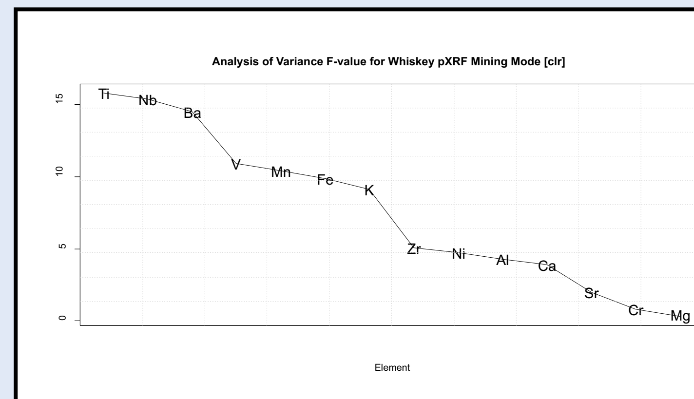
Figure 14. Analysis of variance F-values for 14 elements used to discriminate between the three kimberlite phases (U1VK, U2VK, U3VK) for the pXRF in Mining Mode.
