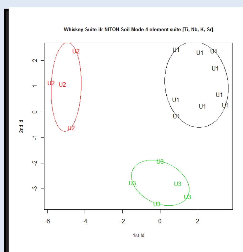
Figure 19. Plot of the first two linear discriminants based on 4 elements (Ti, Nb, K and Sr) for the three kimberlite phases (U1VK, U2VK, U3VK) for the pXRF used in Soil Mode.
