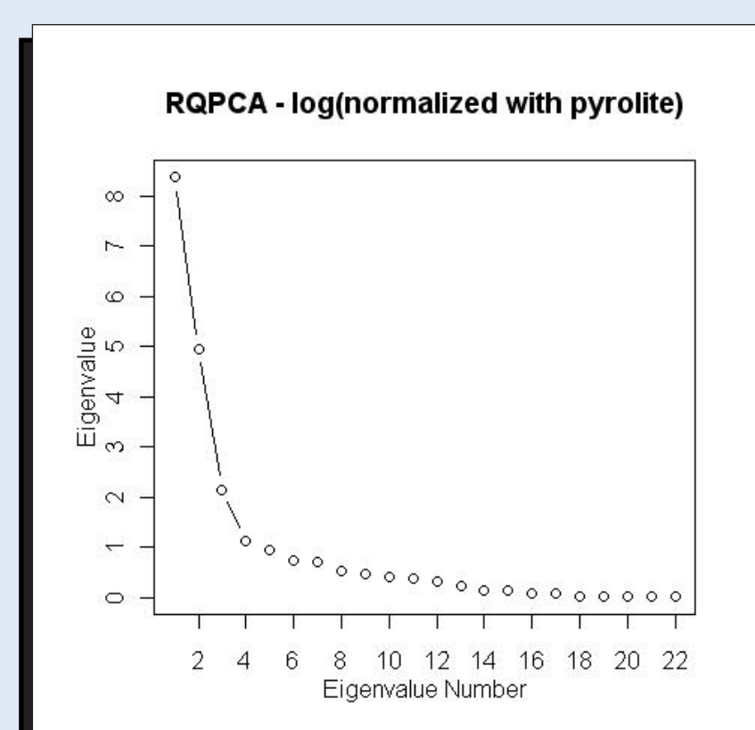
Figure 4. Screeplot of the eigenvalues obtained from a principal component analysis, whole rock data.
