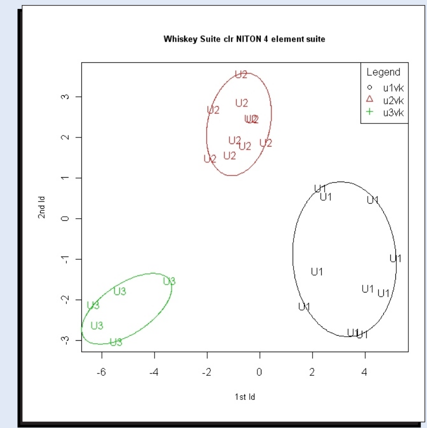
Figure 9. Plot of the first two linear discriminants based on 4 elements (Al, Ti, Cu and Nb) for the three kimberlite phases (U1VK, U2VK, U3VK), calibrated Niton pXRF data.
