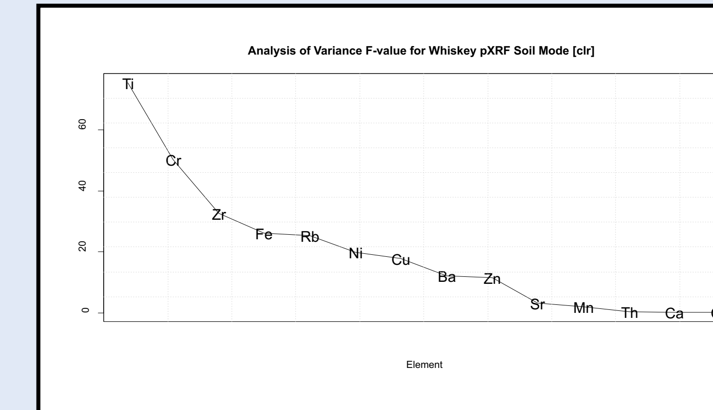
Figure 15. Analysis of variance F-values for 14 elements used to discriminate between the three kimberlite phases (U1VK, U2VK, U3VK) for the pXRF in Soil Mode.
