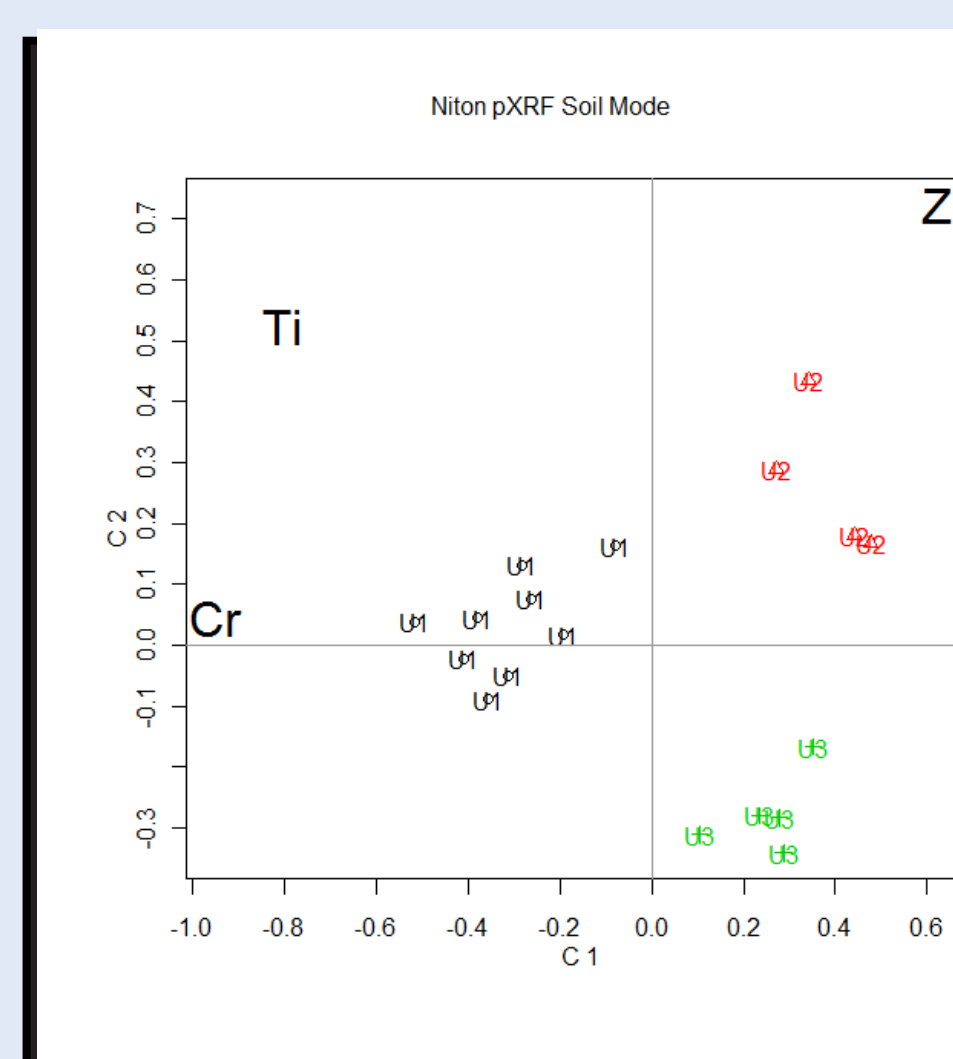
Figure 17. Biplot of the first two principal components of the Whiskey kimberlite phases based on 3 elements for the pXRF in Soil Mode.
