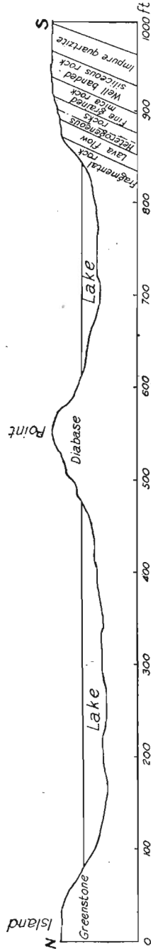
Figure 1. Section showing relation of lower and upper divisions of the Pre-Granite Complex, Knee Lake, Manitoba.
