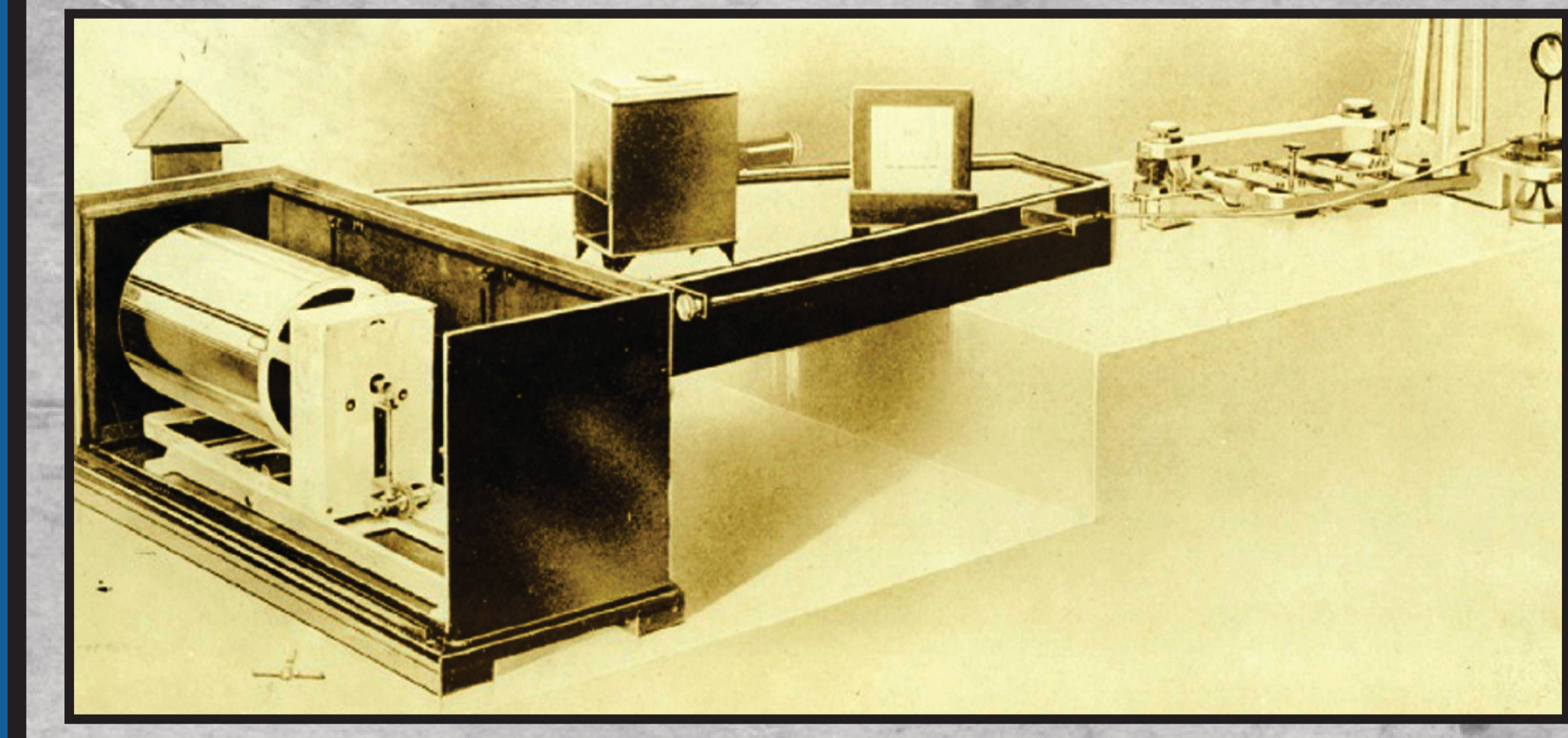
A seismograph of the same type as those in operation at the Dominion Observatory at Ottawa in 1925
