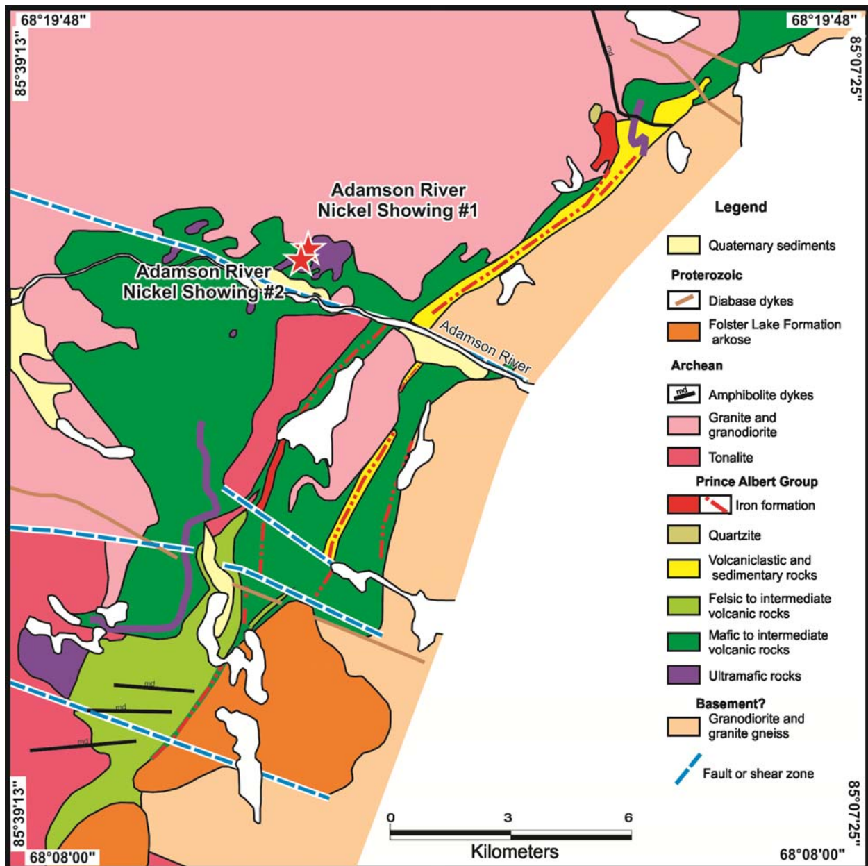
Figure 3. Simplified geological map of the southern part of the Prince Albert greenstone belt of the Melville Peninsula showing the main lithologies and the location of the two Adamson River nickel showings in the Prince Albert Hills (modified after Frisch, 1982).
