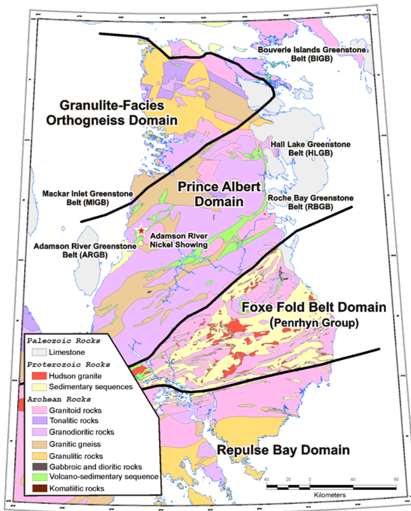
Figure 2. Geological overview of the Melville Peninsula showing the four main lithotectonic entities and the location of the Adamson River showing in the Prince Albert Hills (modified from Skulski, in prep.).
