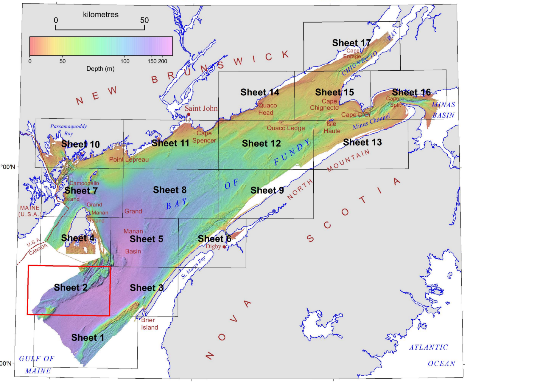
Figure 1. Location map showing seventeen 1:50 000 map sheets covering the Bay of Fundy. Sheet 2 (outlined by red line) is southernmost Bay of Fundy south of Grand Manan Island, New Brunswick.
