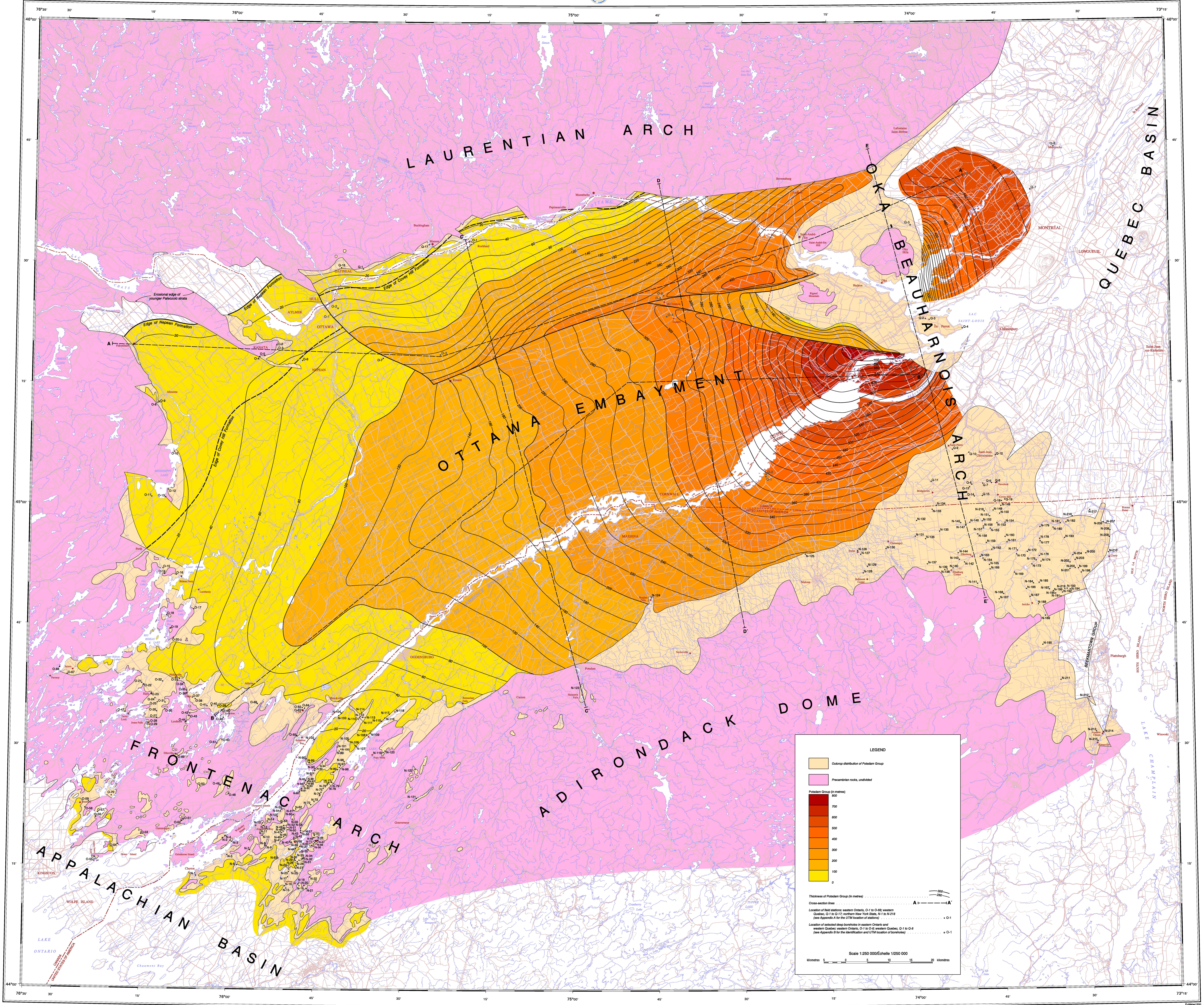
Figure 6. Isopach map showing the distribution and thickness of the Potsdam Group and the locations of sections where the rocks are best exposed in eastern Ontario, western Quebec, and northern New York State.
